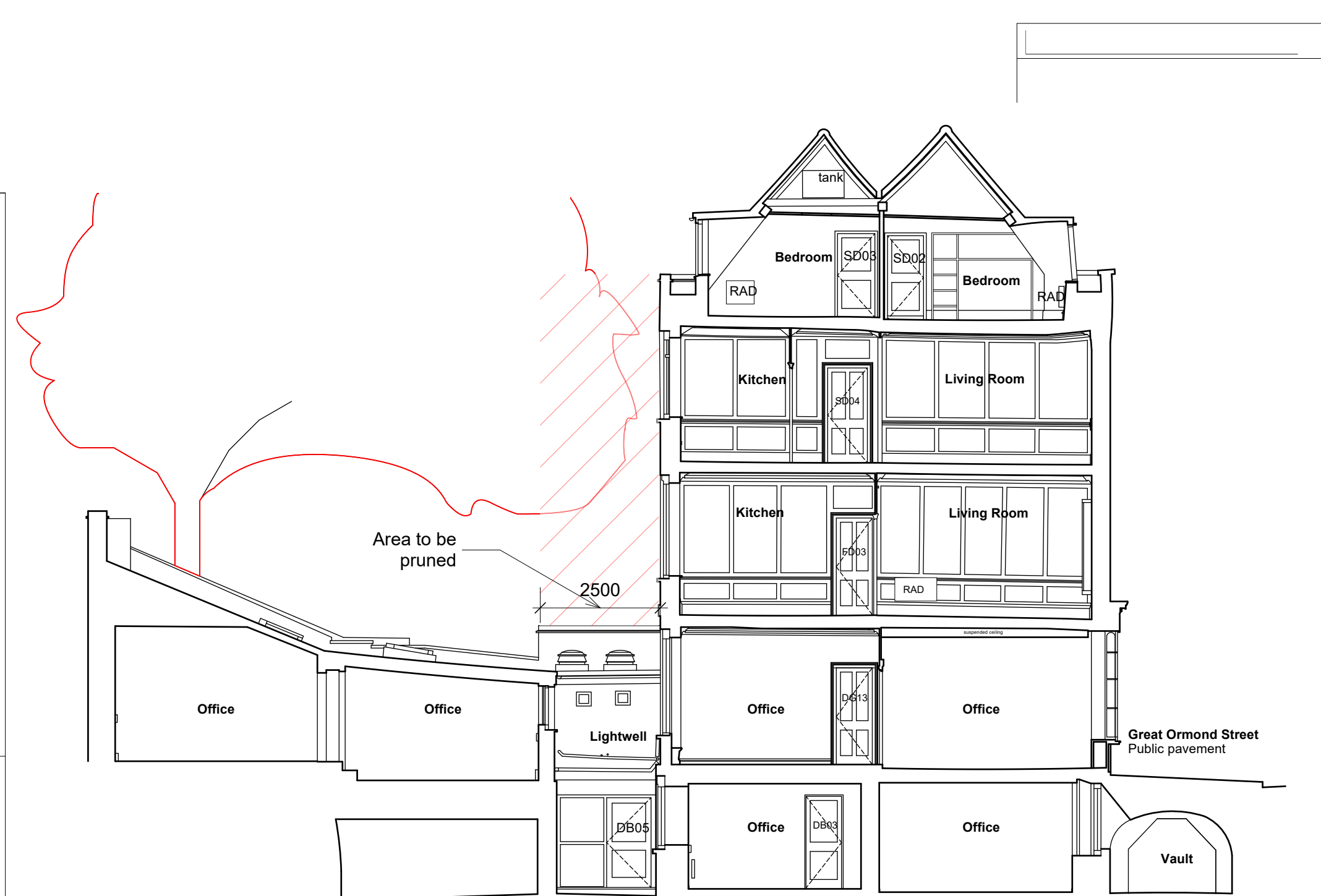
Section through 51 Great Ormond Street, showing location of tree (red outline)
