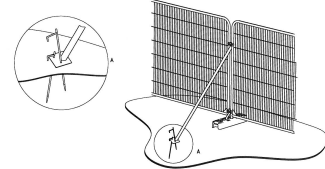
Figure 2 Examples of above-ground stabilizing systems
