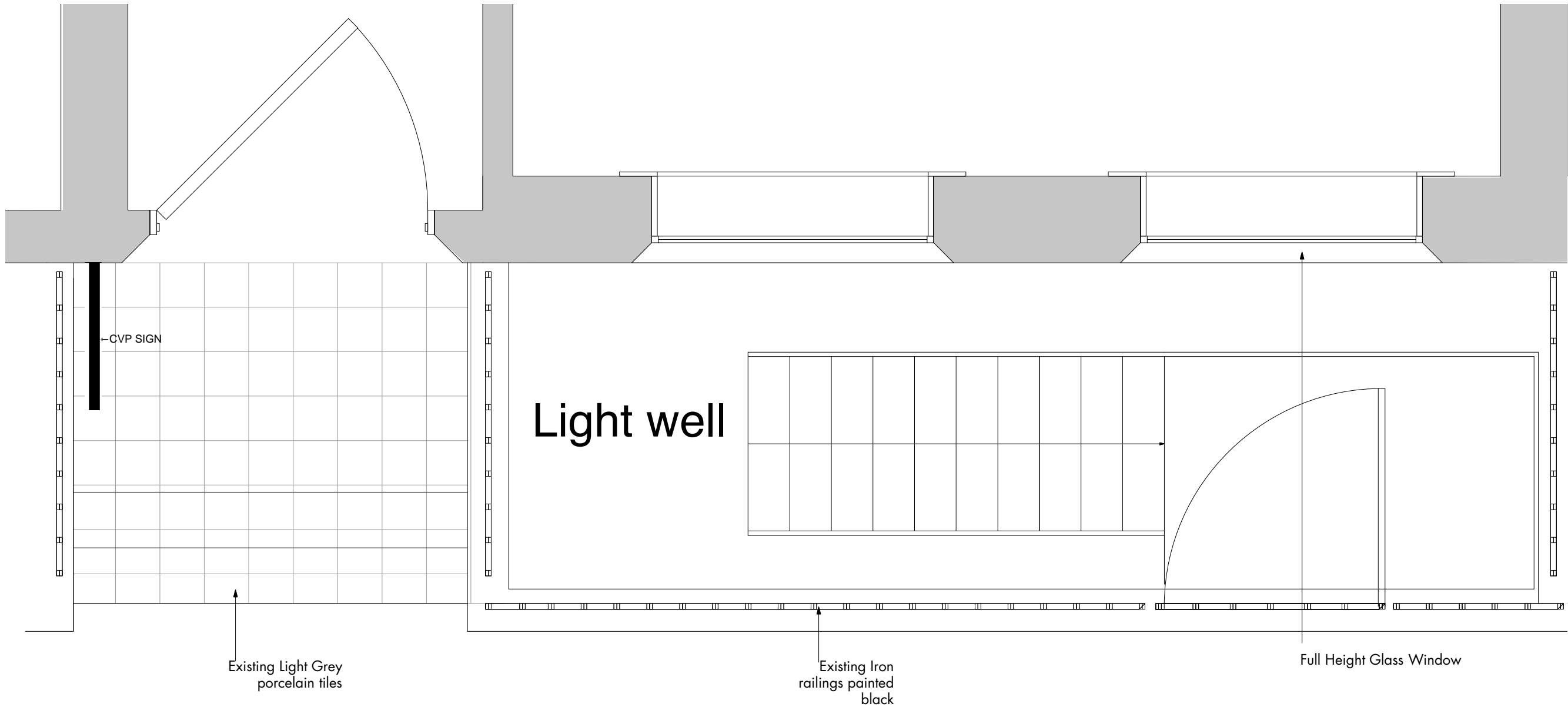
1 Existing Entrance Steps 1:20 @A3
