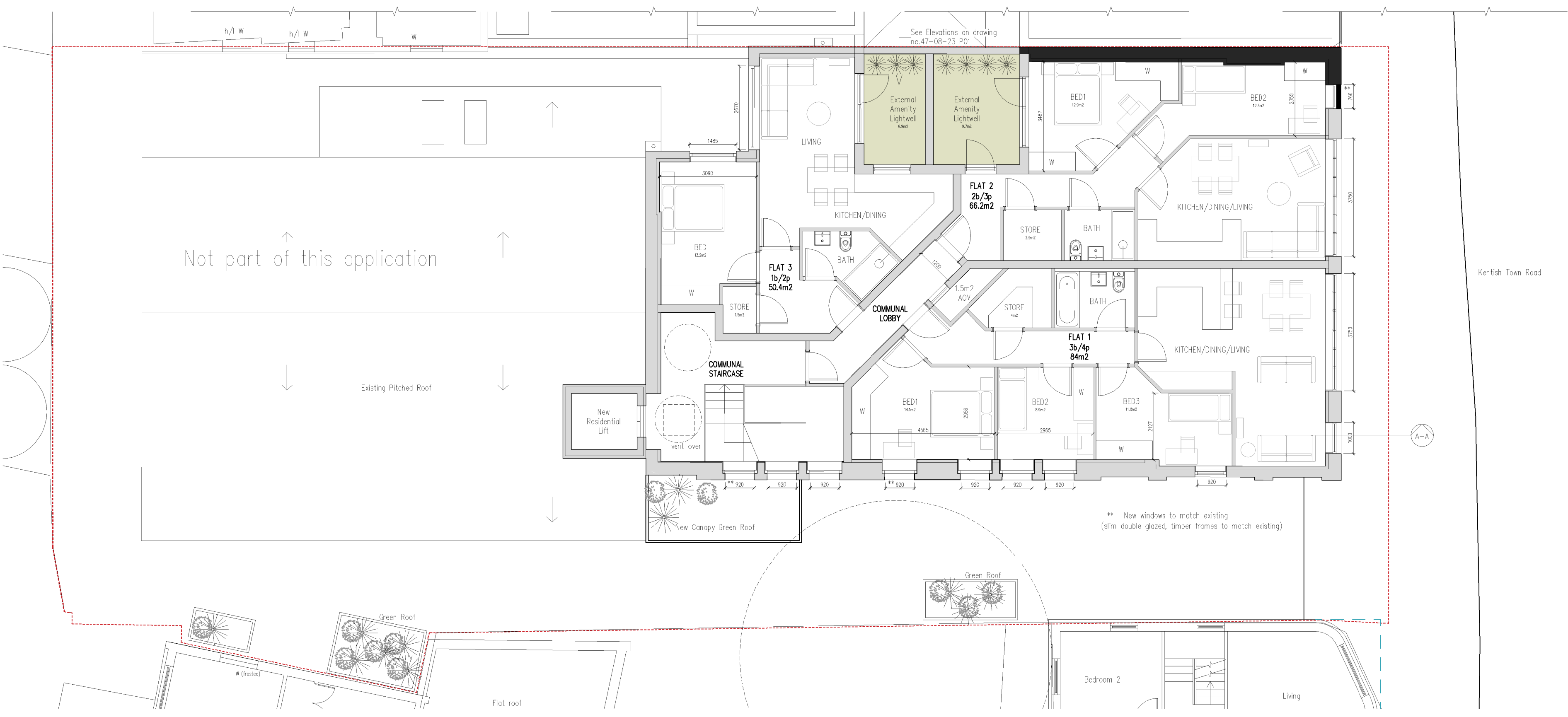
Proposed First Floor Plan, 1:200
