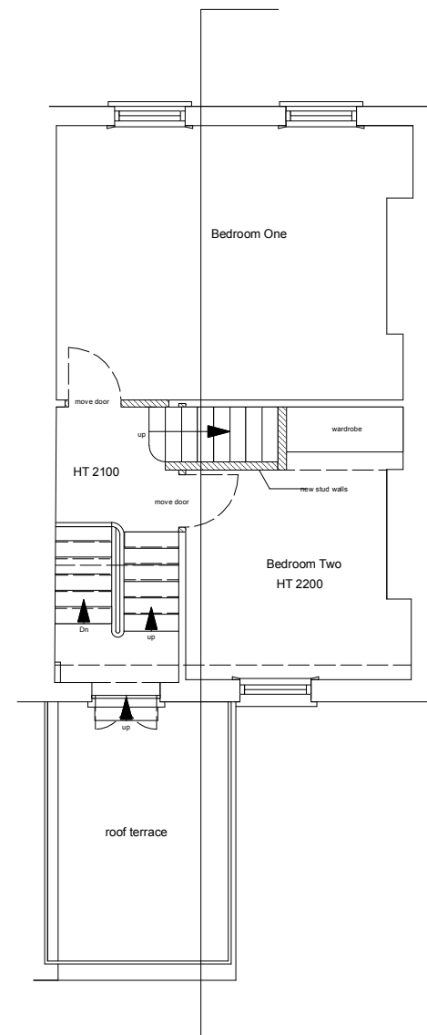
Proposed Second Floor Plan
