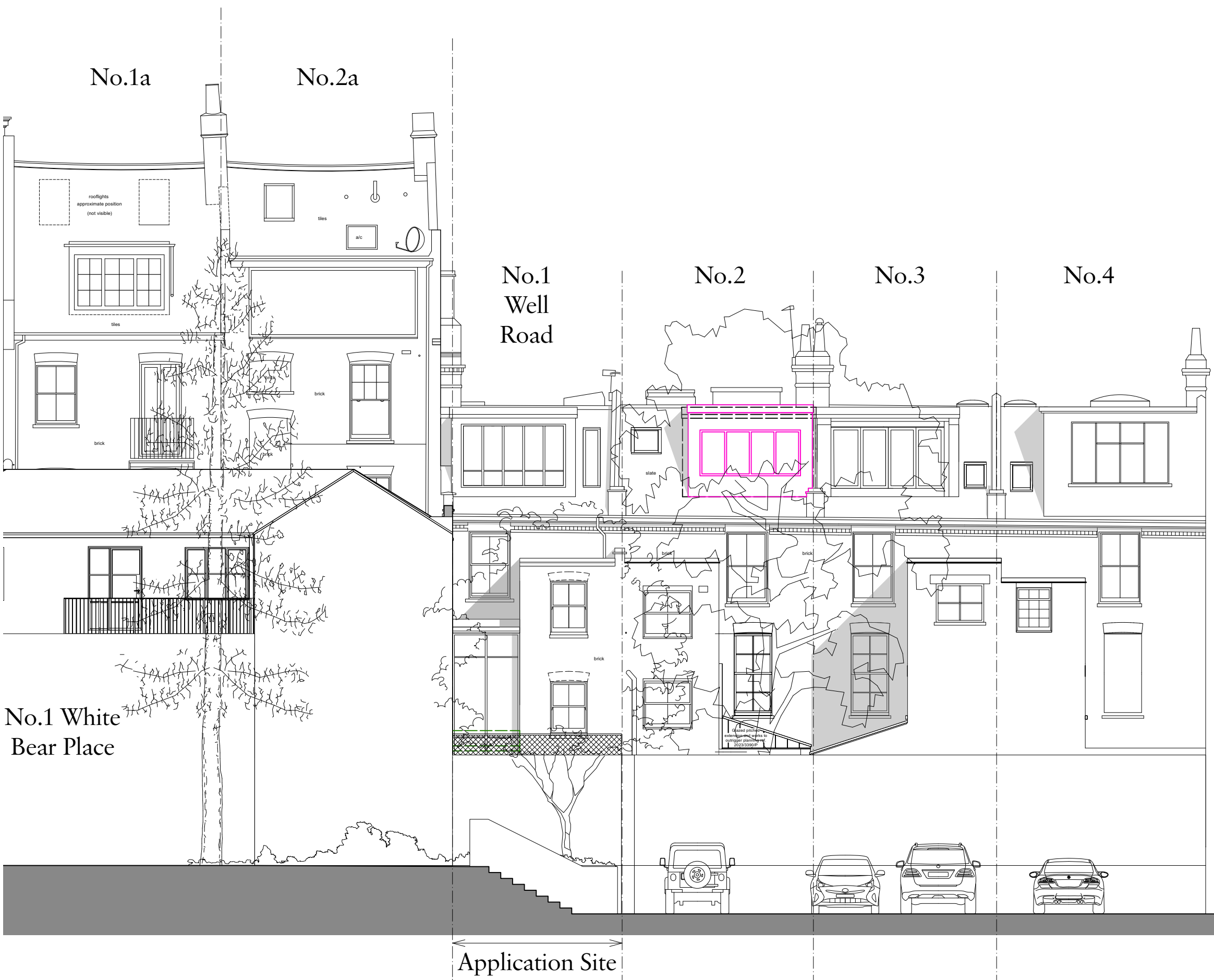
2 Proposed South East Elevation Scale: 1:100
