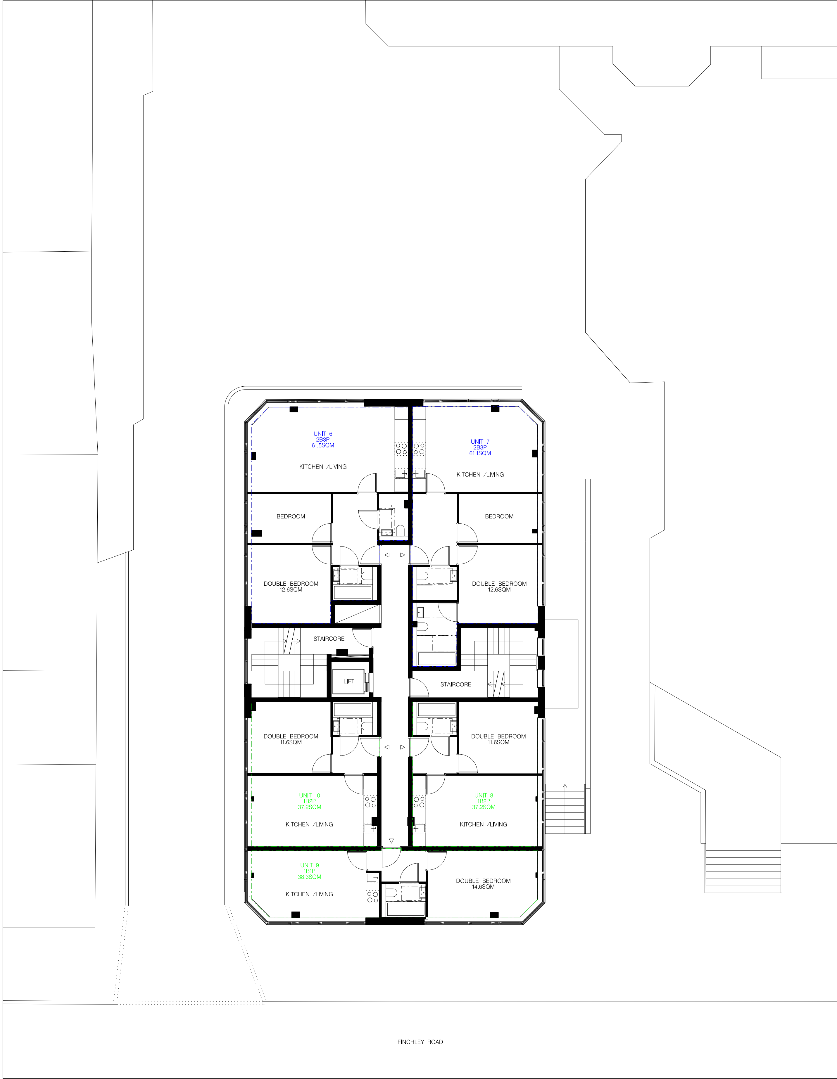
1 PROPOSED CLASS MA FIRST FLOOR PLAN
