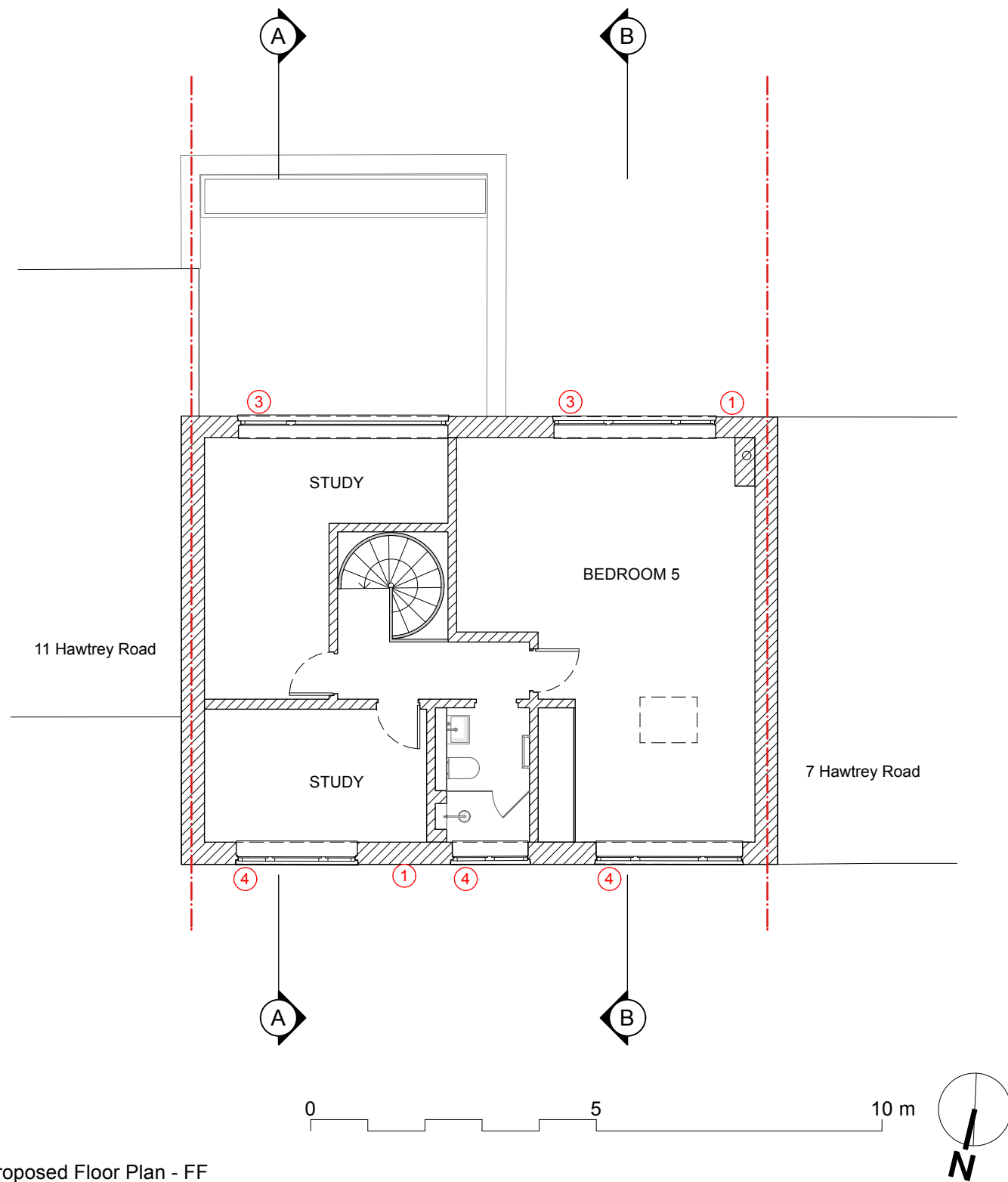
3 Proposed Floor Plan - FF Scale: 1:100
