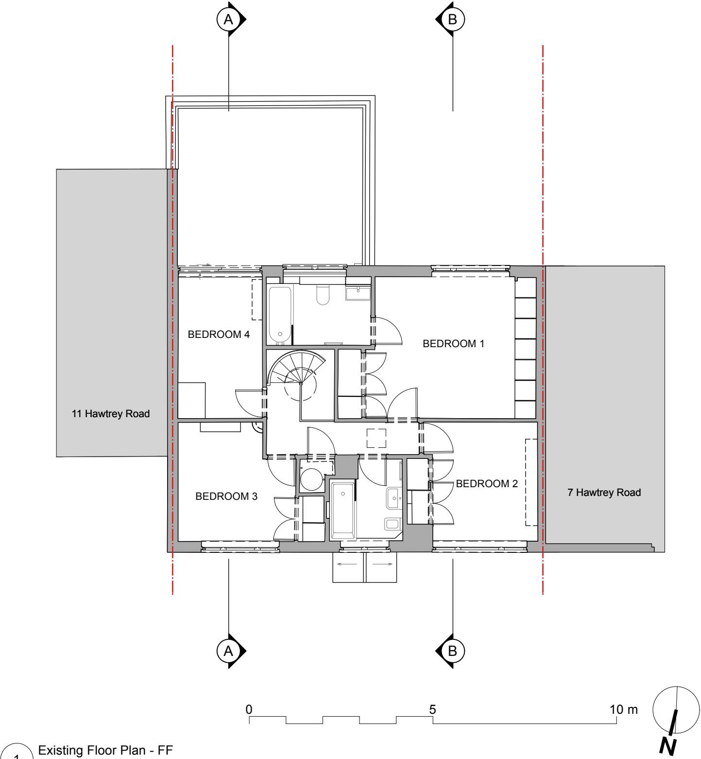
1 Existing Floor Plan - FF Scale: 1:100
