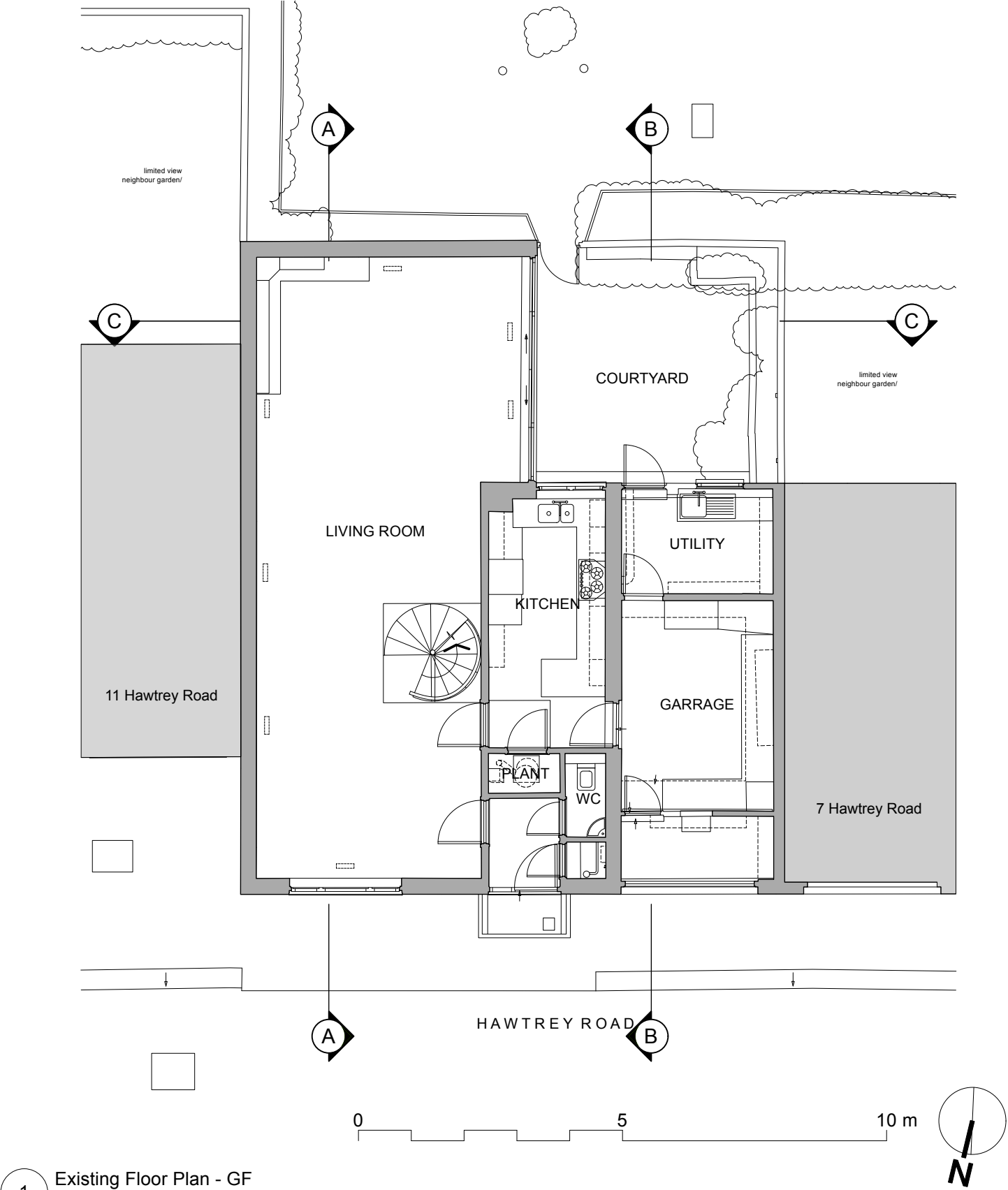
1 Existing Floor Plan - GF Scale: 1:100
