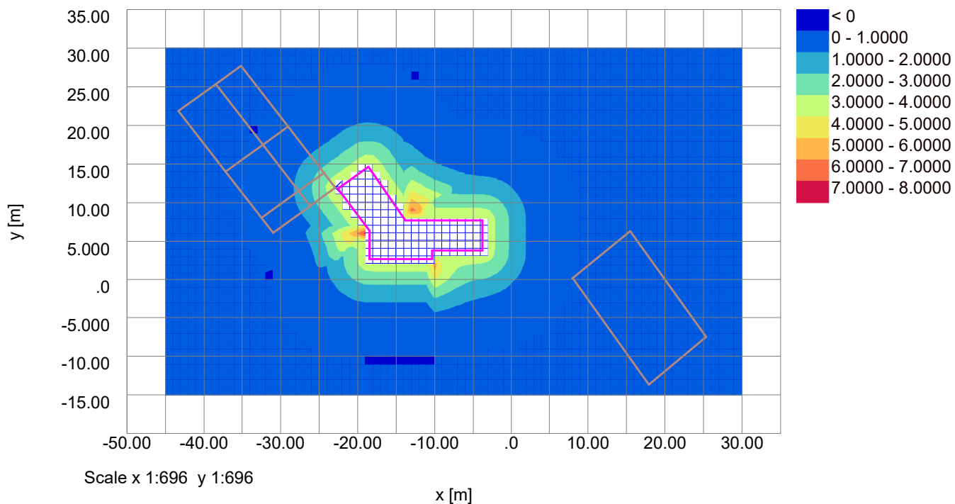
Vertical Settlement Contours: Grid 1 (level 99.300m) (Interval 1mm)
