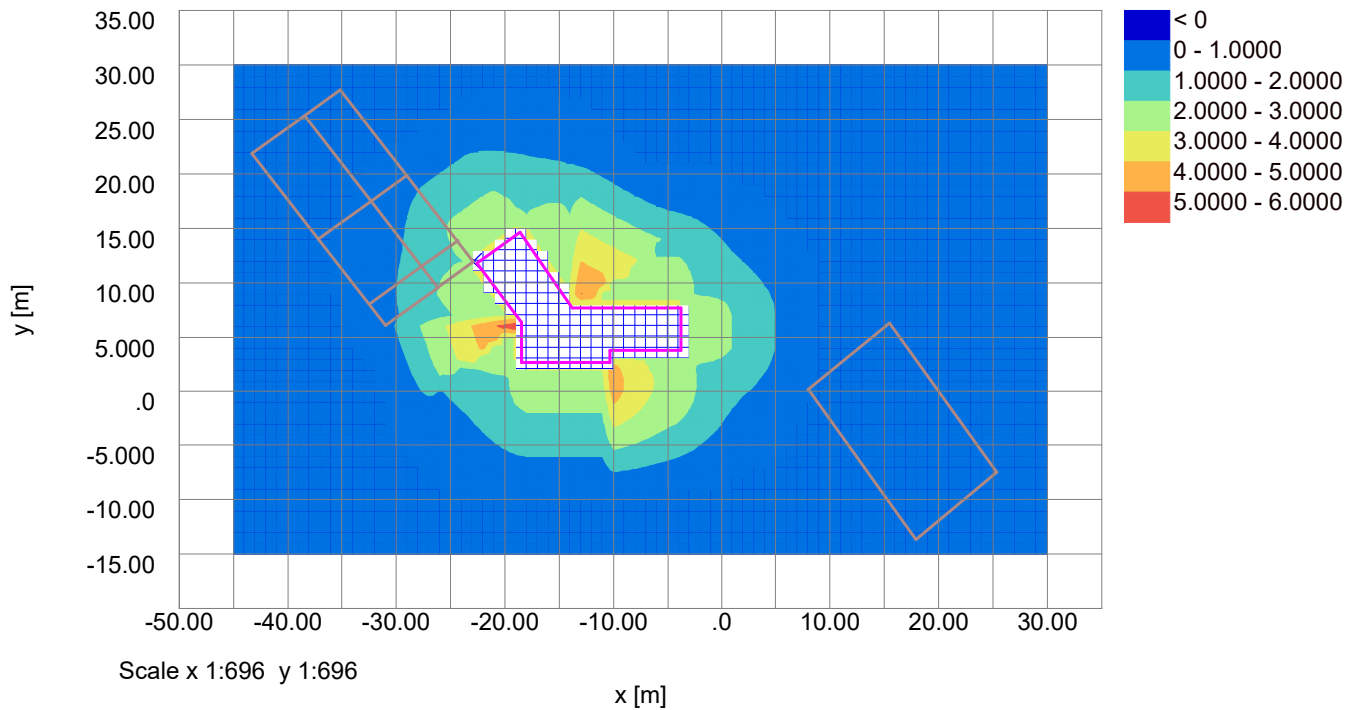
Horizontal Displacement Contours: Grid 1 (level 99.300m) Interval 1mm
