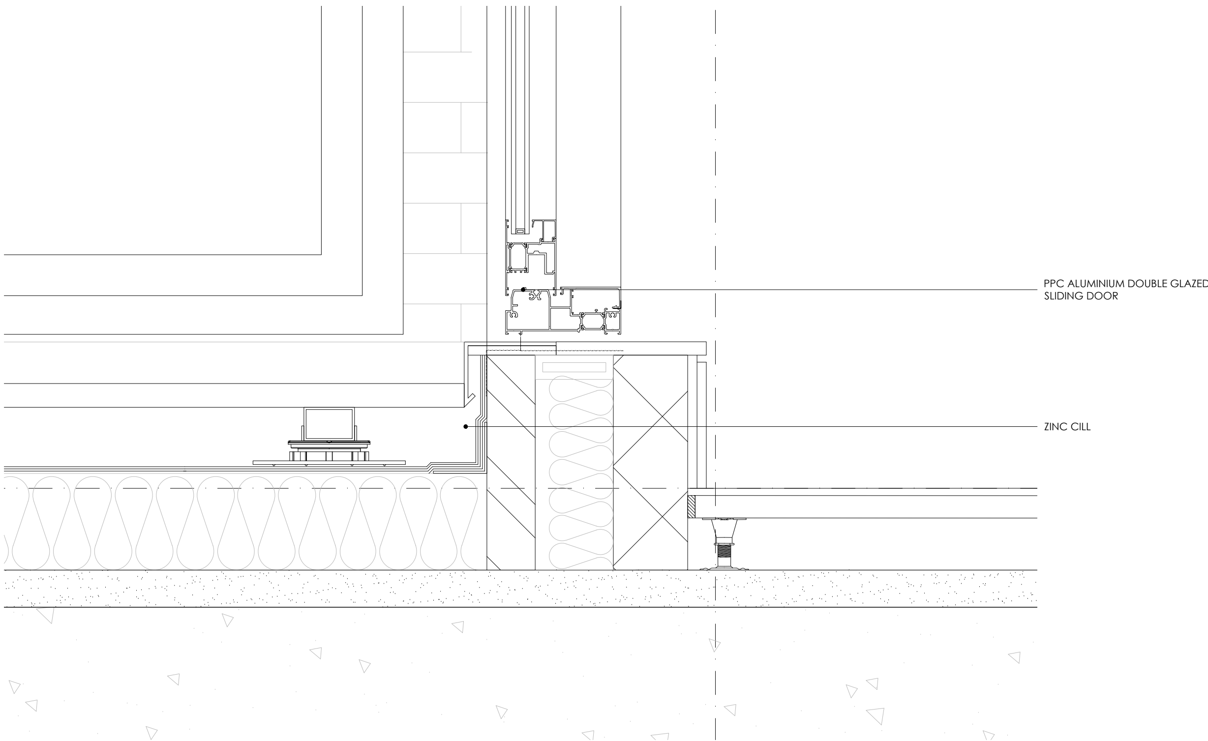
4. PROPOSED 6FL SLIDING DOOR BASE DETAIL
