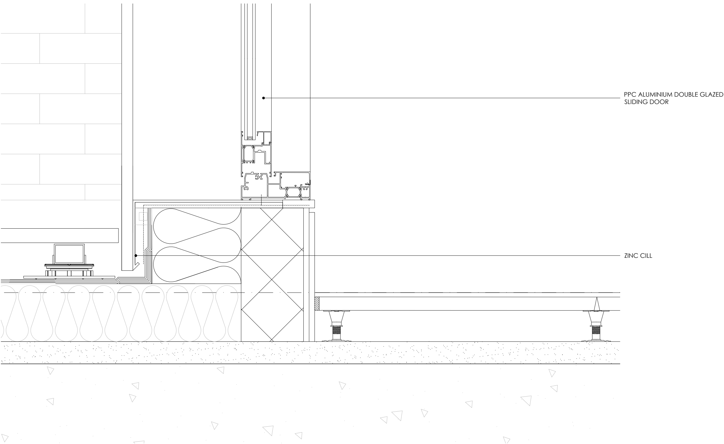
3. PROPOSED 5FL DORMER BASE DETAIL
