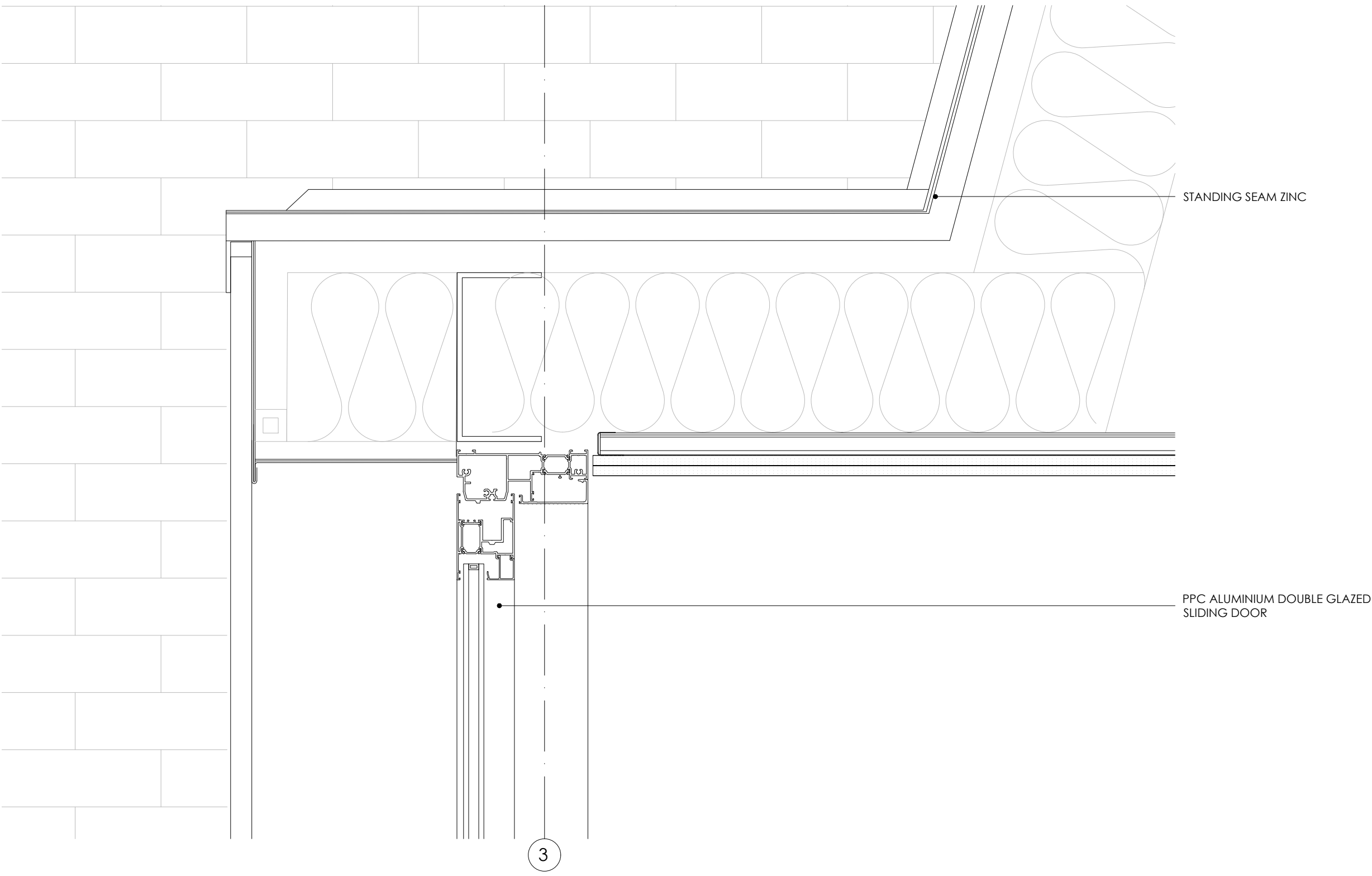
1. PROPOSED 5FL DORMER HEAD DETAIL
