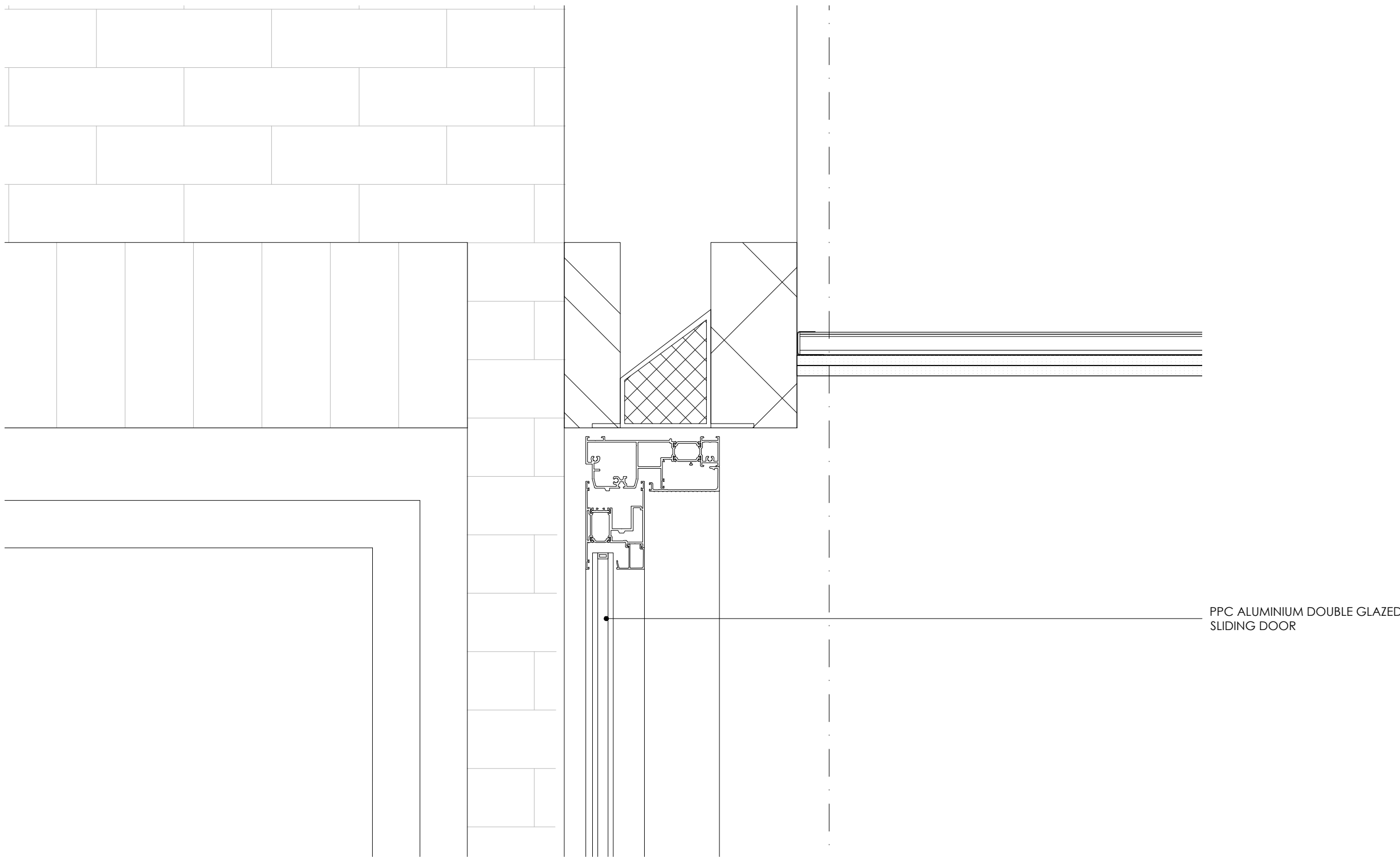
2. PROPOSED 6FL SLIDING DOOR HEAD DETAIL
