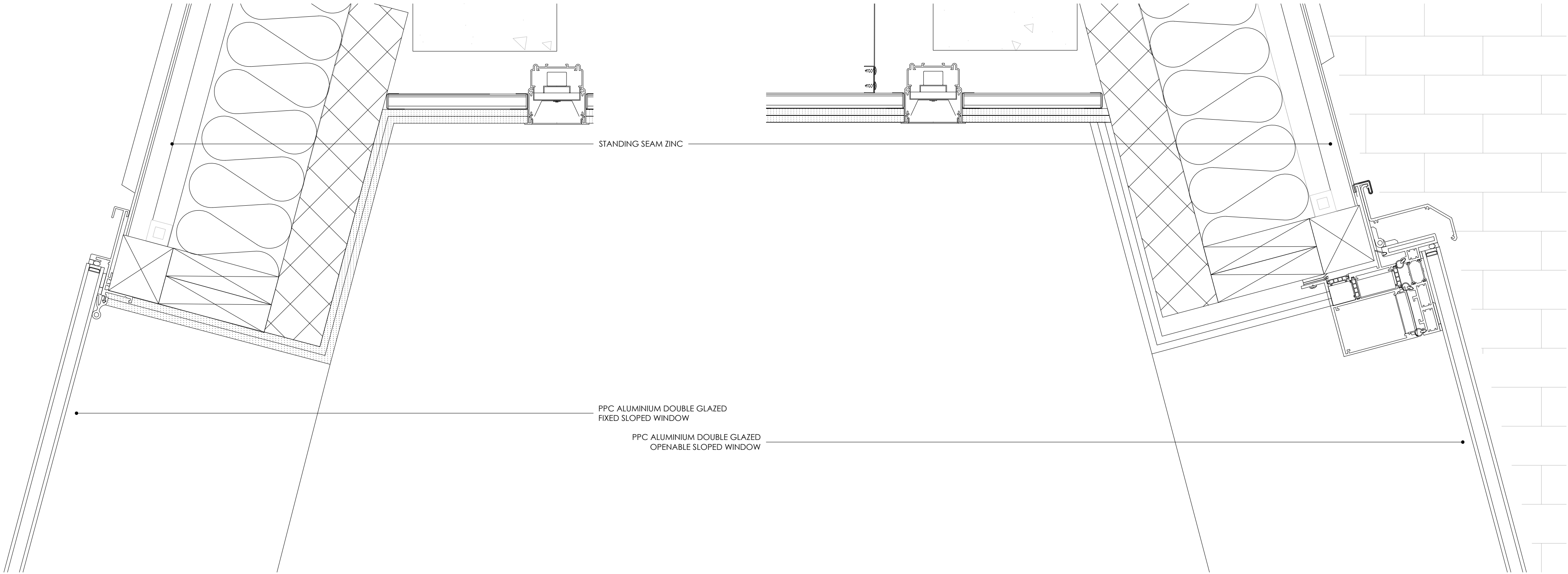
1. PROPOSED SLOPED WALL FIXED WINDOW HEAD DETAIL
