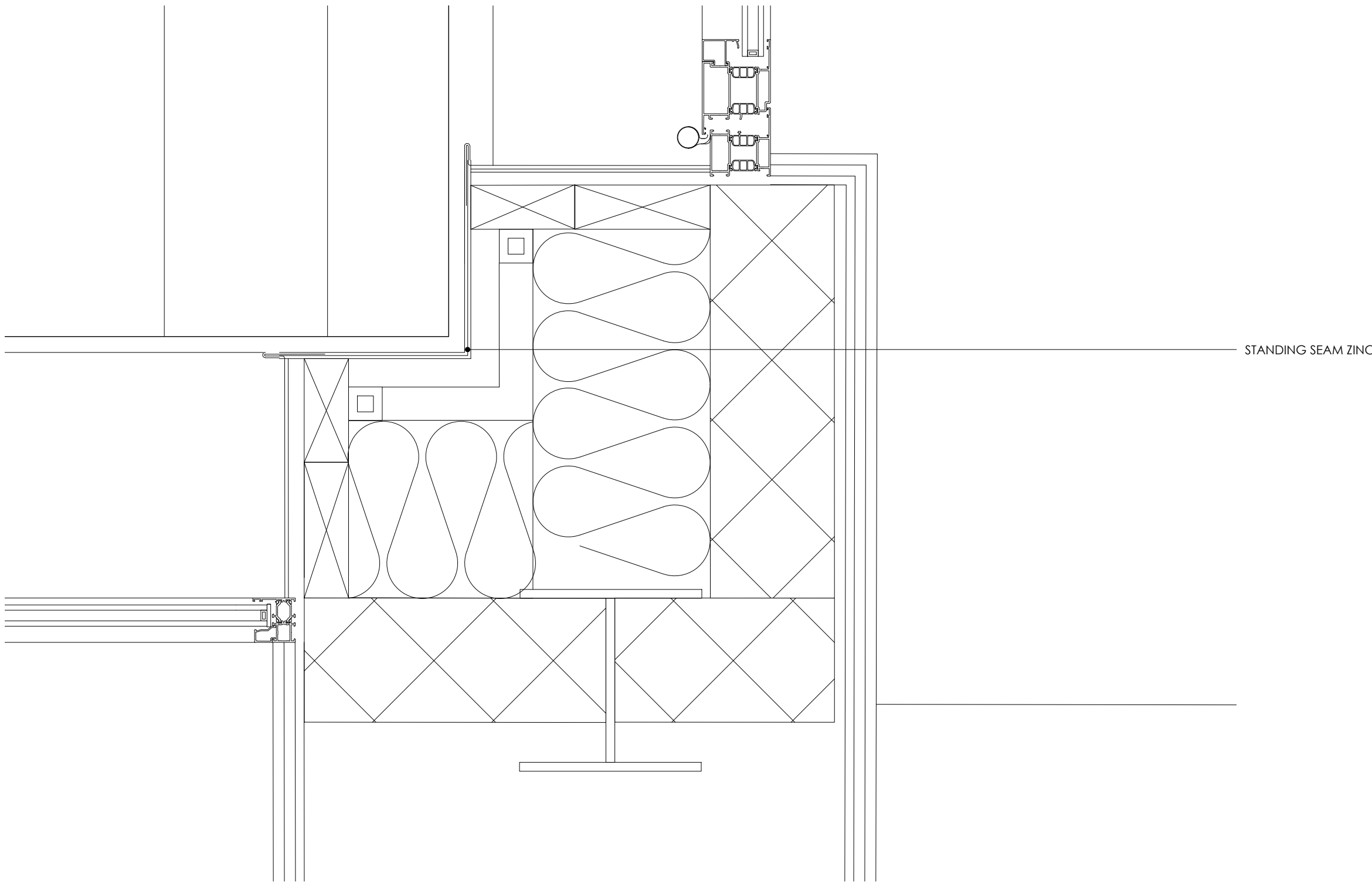
2. PROPOSED SLOPED WALL INTERNAL CORNER DETAIL
