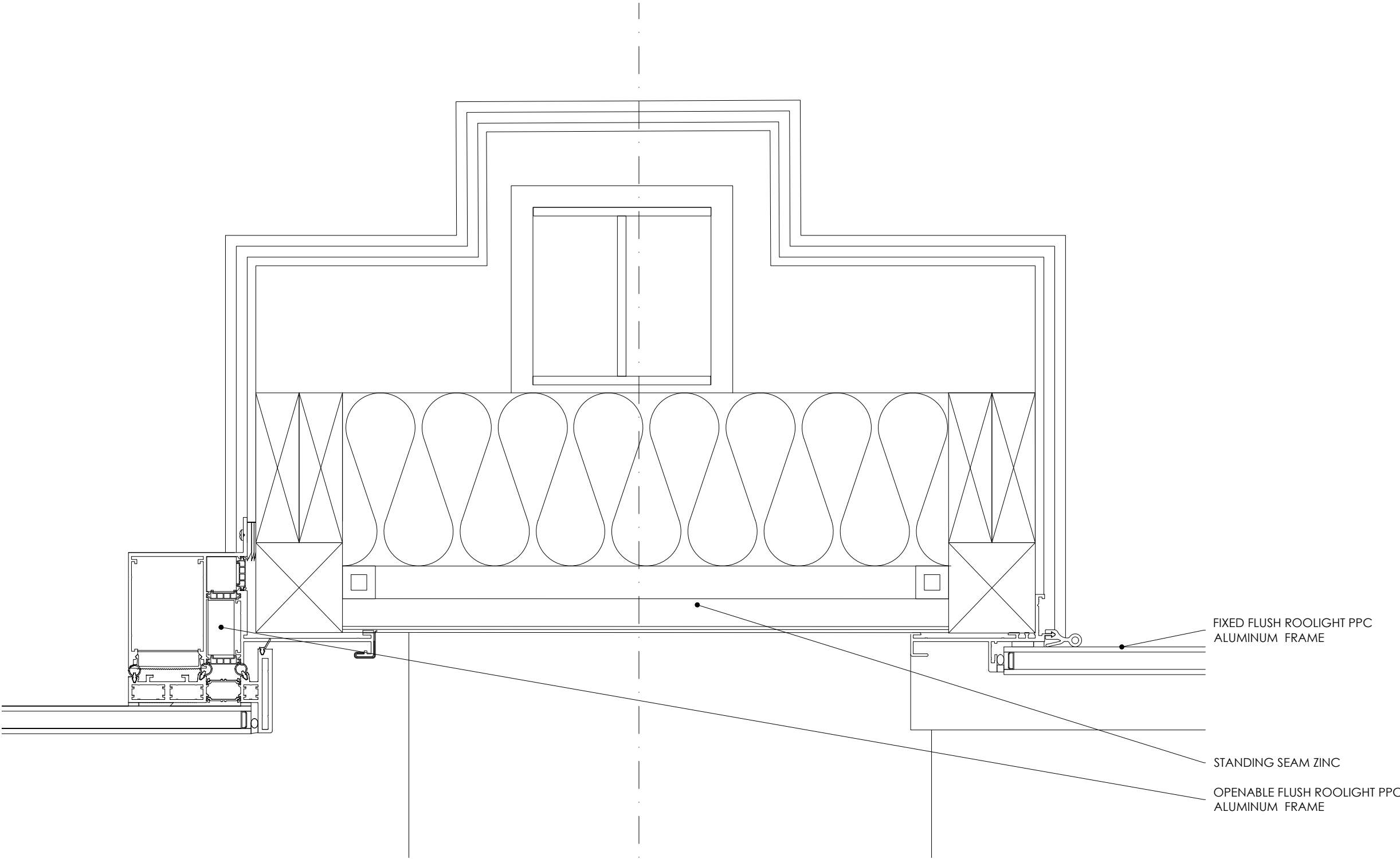
4. PROPOSED SLOPED WALL TO WINDOW JAMB DETAIL
