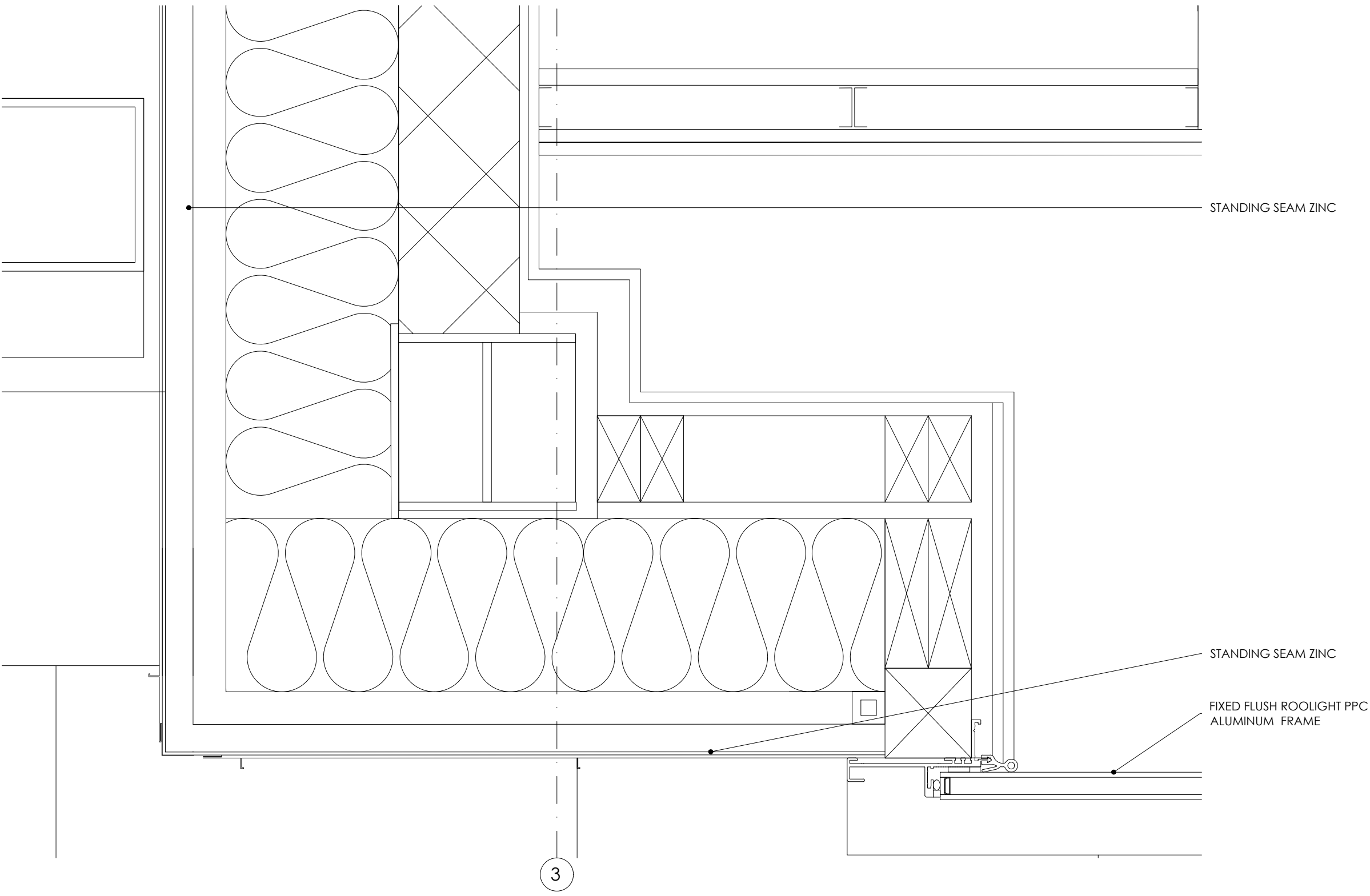
1. PROPOSED SLOPED WALL EXTERNAL CORNER DETAIL
