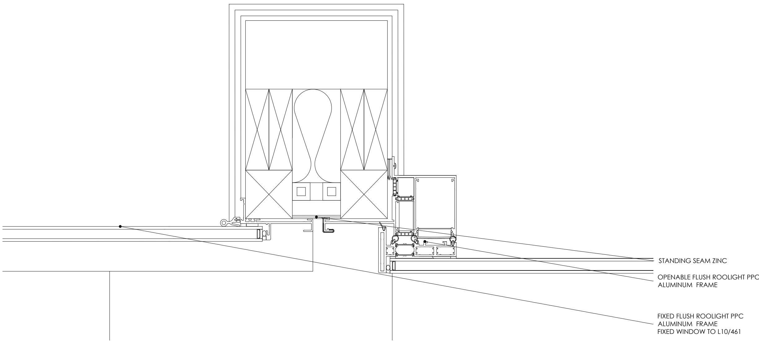
4. PROPOSED SLOPED WALL TO WINDOW JAMB DETAIL
