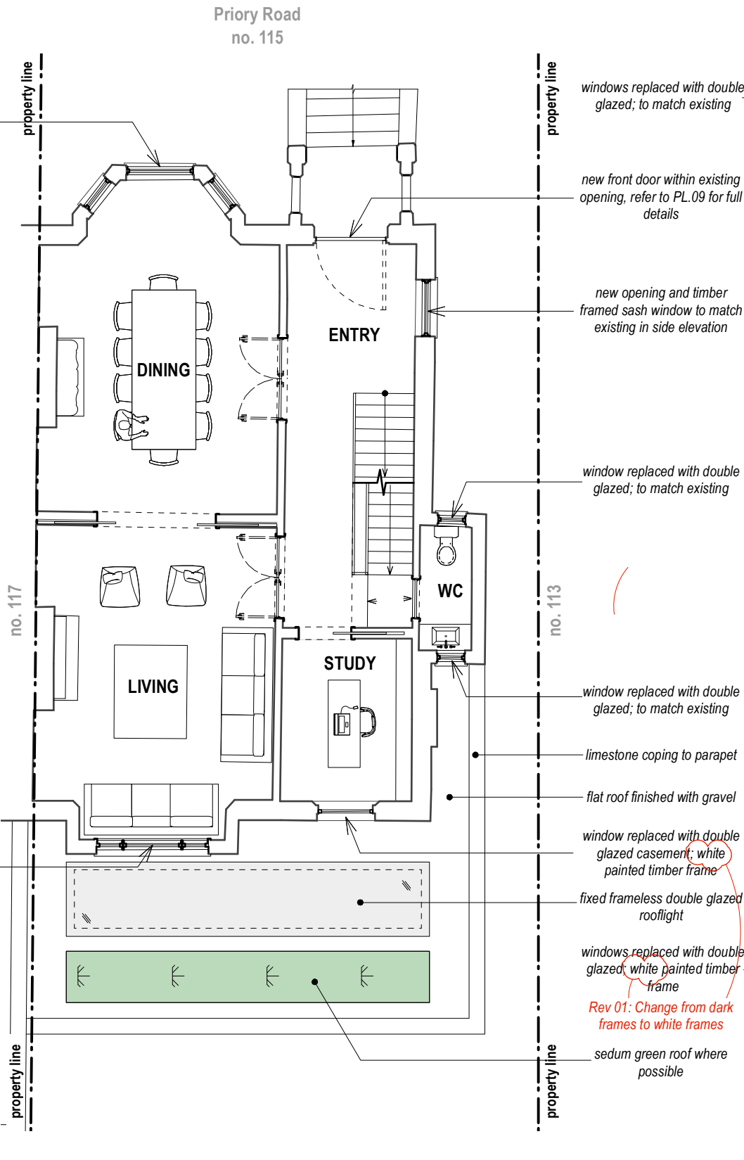
2 PROPOSED UPPER GROUND FLOOR 1:100 @ A3
