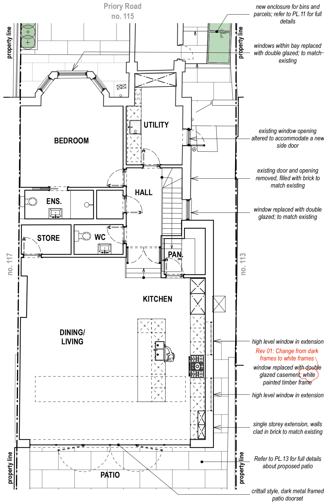
1 PROPOSED LOWER GROUND FLOOR 1:100 @ A3
