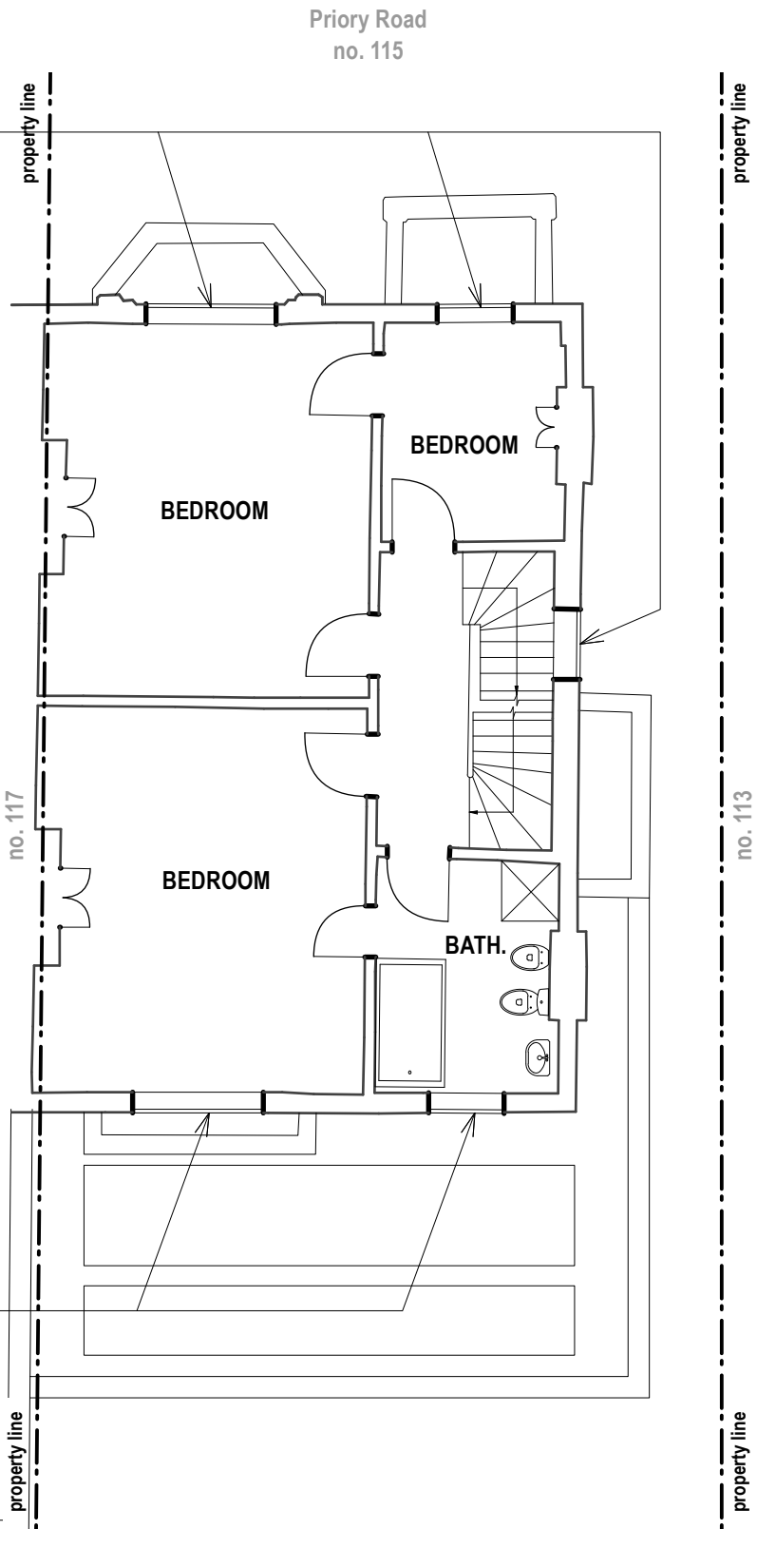
3 PROPOSED FIRST FLOOR 1:100 @ A3
