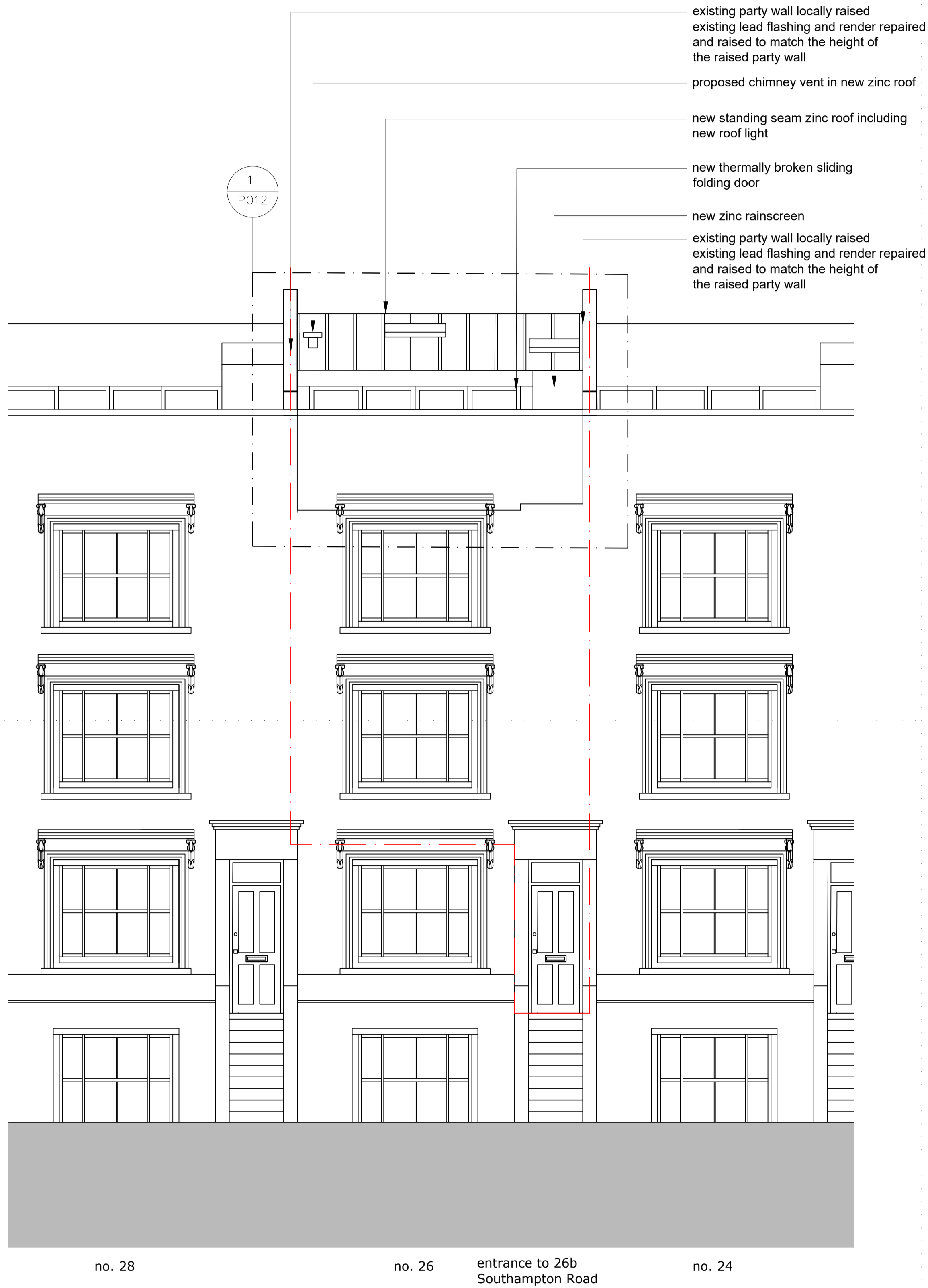
Front elevation
