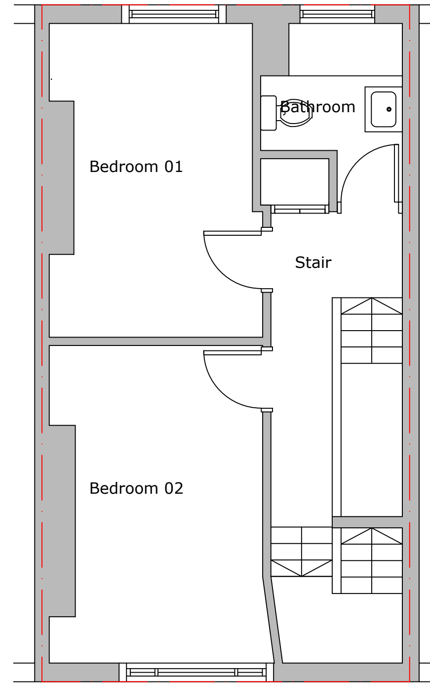
First floor
