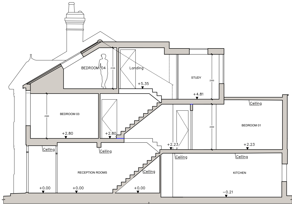
1 Existing Section LDC # 2025/1005/P
