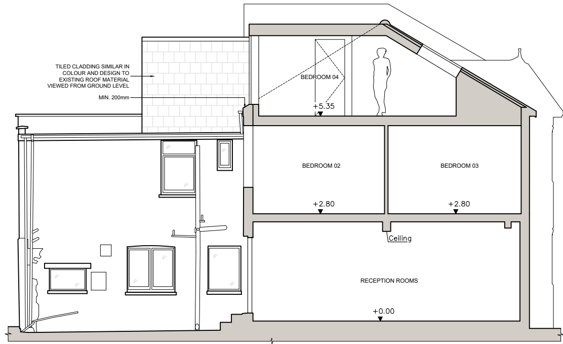
2 Existing Section LDC # 2025/1005/P
