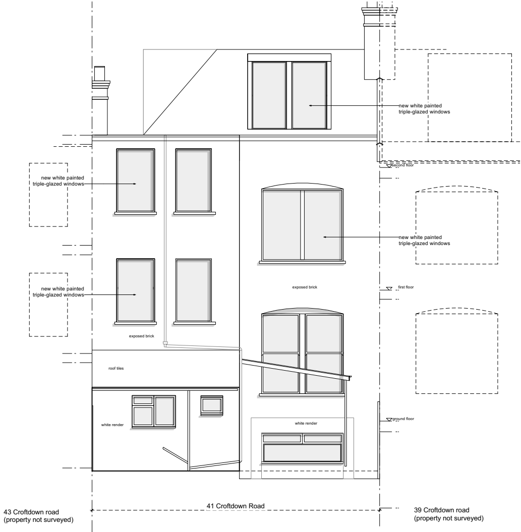
REAR ELEVATION
