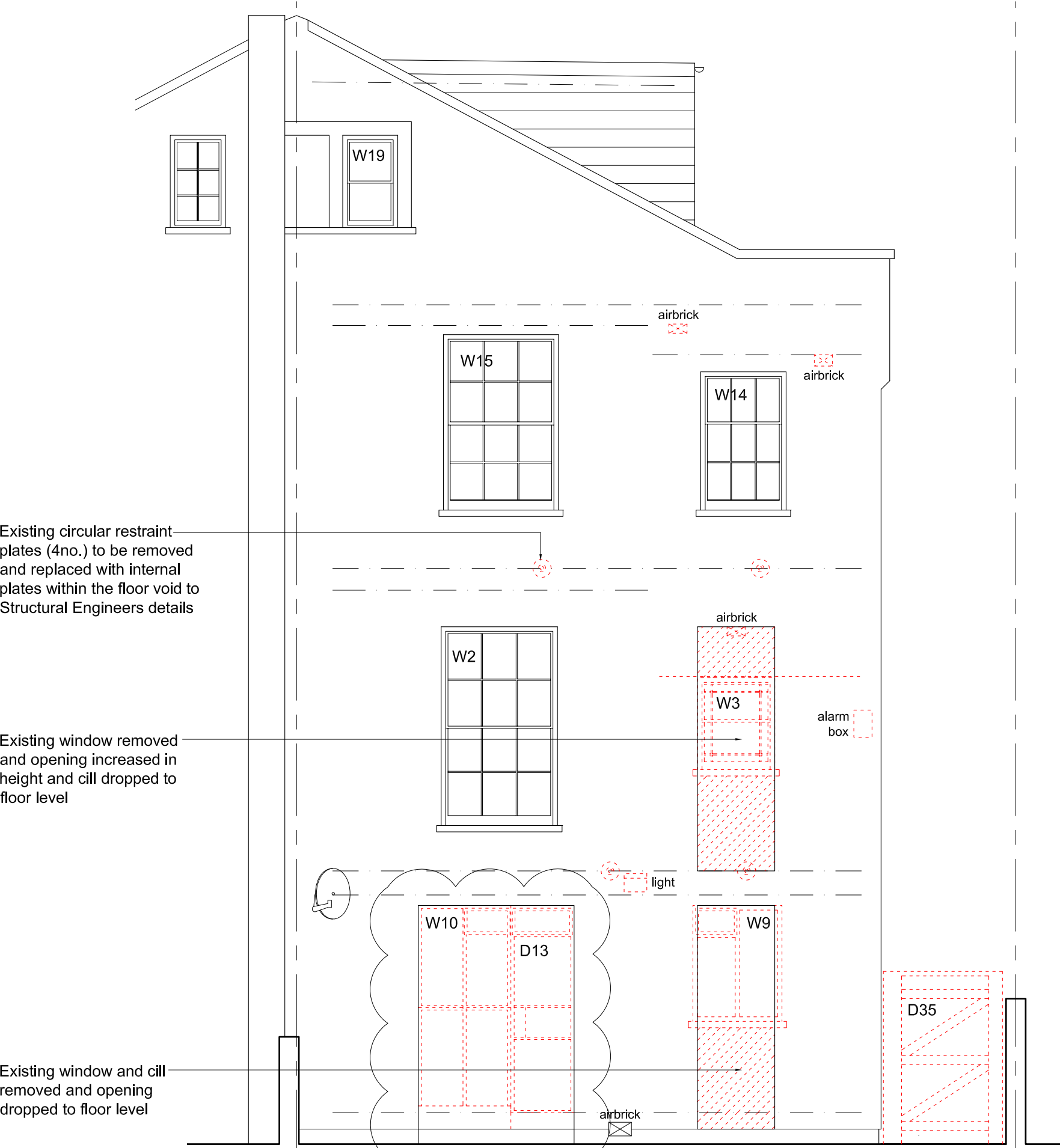
Rear Elevation as Existing - Downtakings Scale 1:50 @ A3
