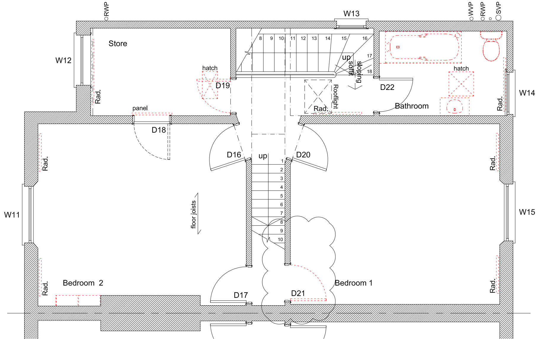
First Floor Plan as Existing - Downtakings
