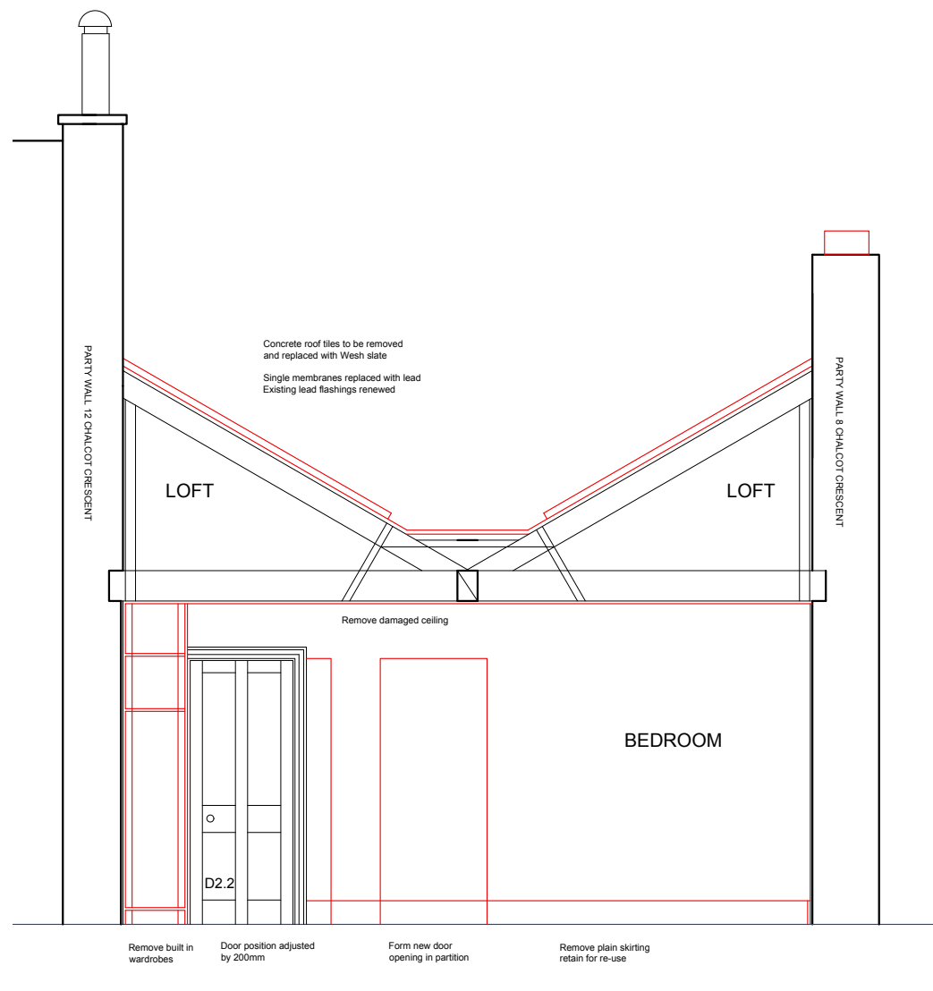
EXISTING BEDROOM ELEVATION
