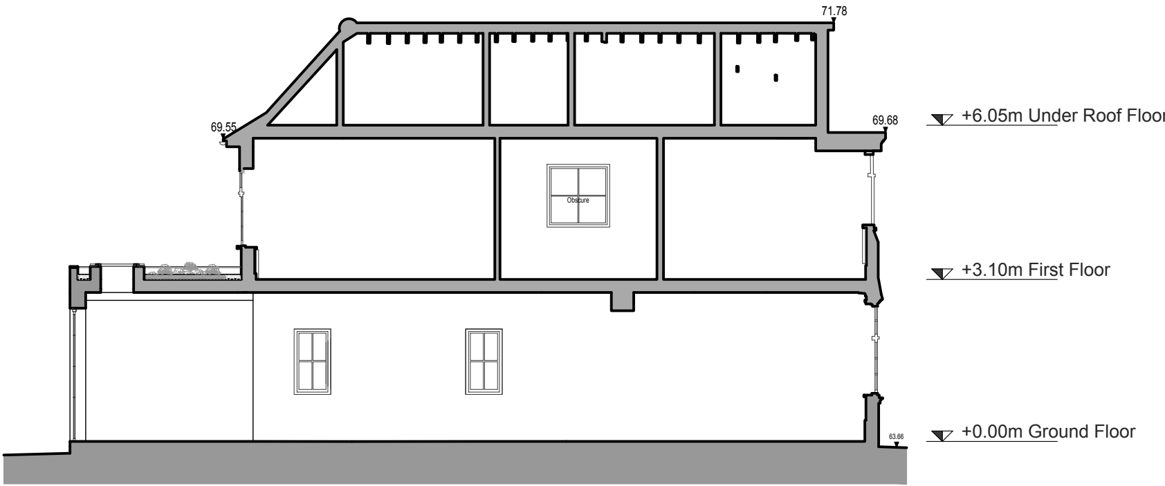
SECTION A
