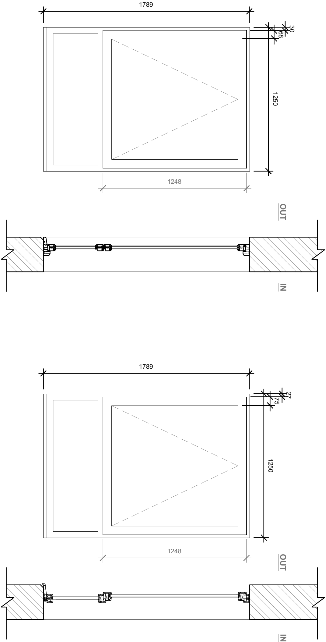
Existing typical Window Elevation Scale 1:20
