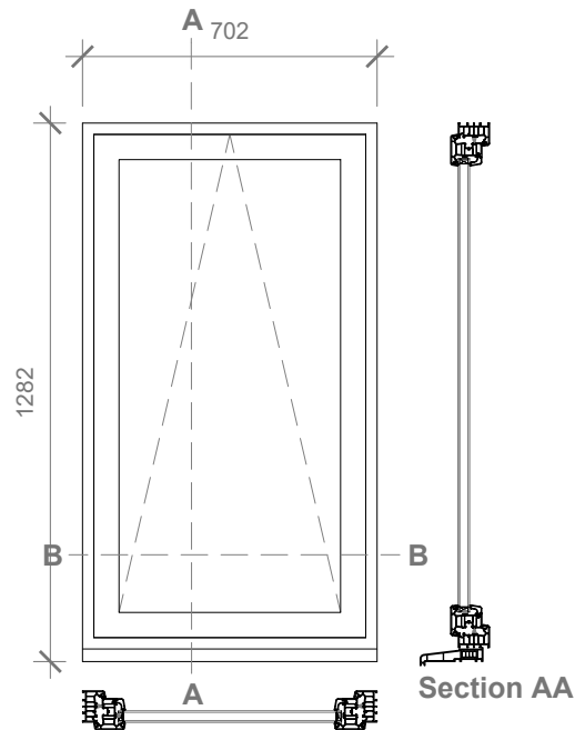
W4 - 702X1282MM Scale 1:20 (Type-3)
