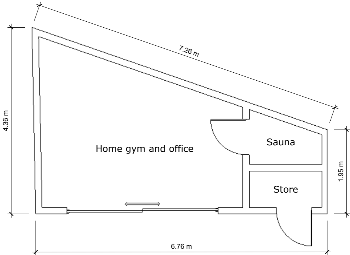
Floor Plan
