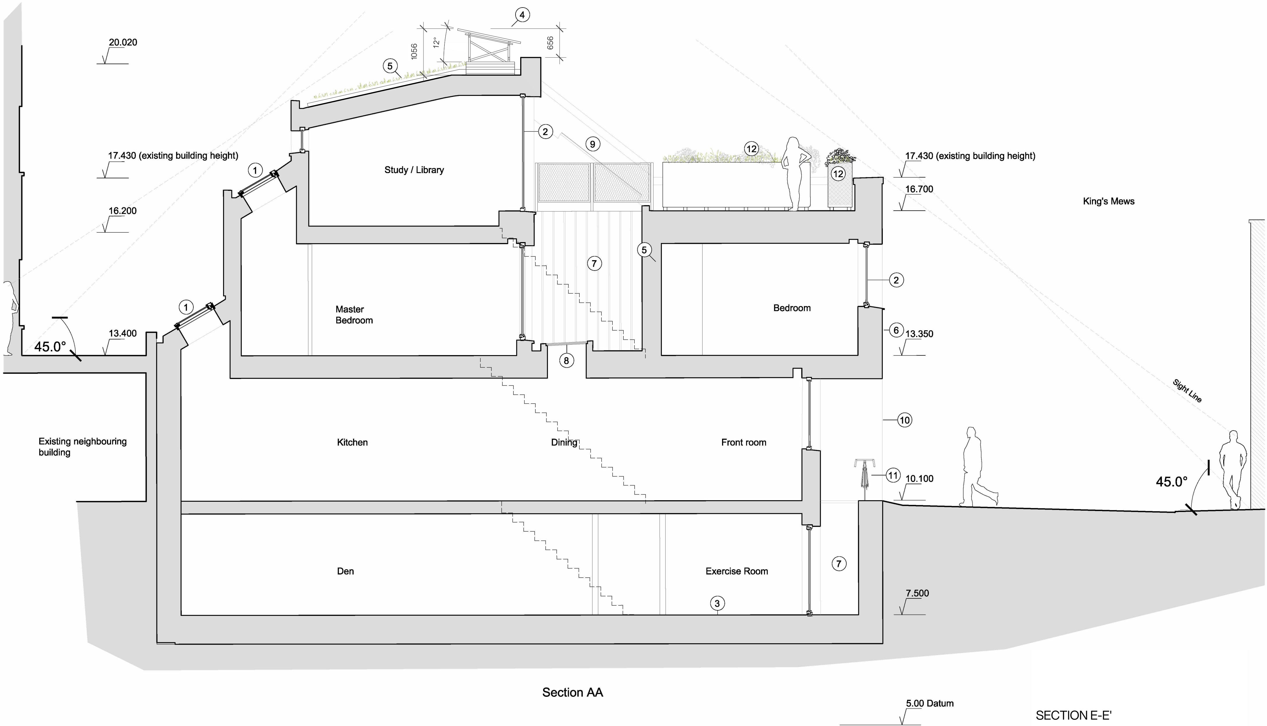
1 Section E-E' - Proposed 1 : 50
