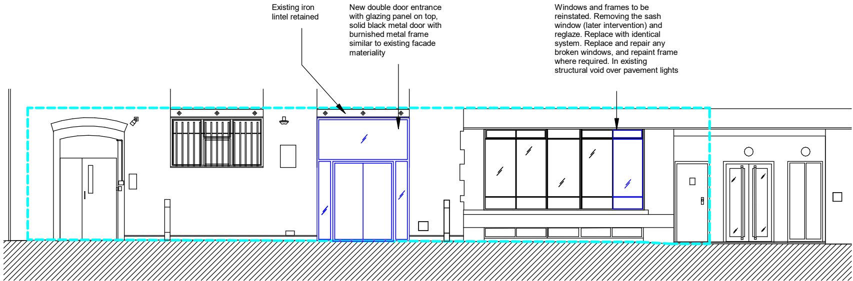
1 Proposed West Elevation - Demise 1 : 100
