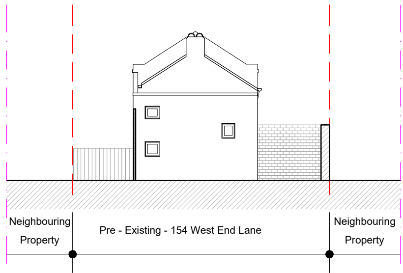
Rear Elevation
