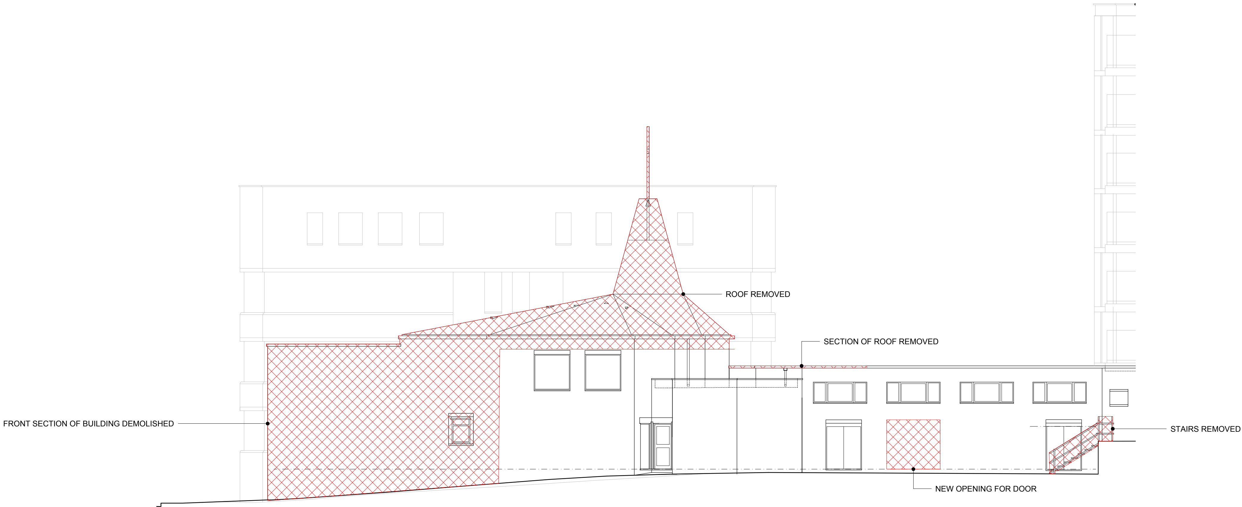
NORTH ELEVATION
