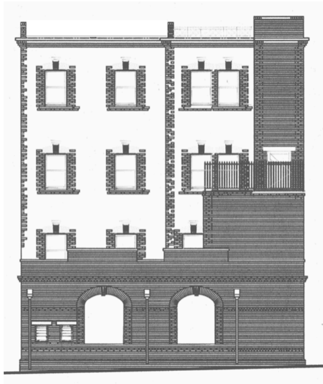
EXISTING EAST ELEVATION TO ROCHESTER PLACE
