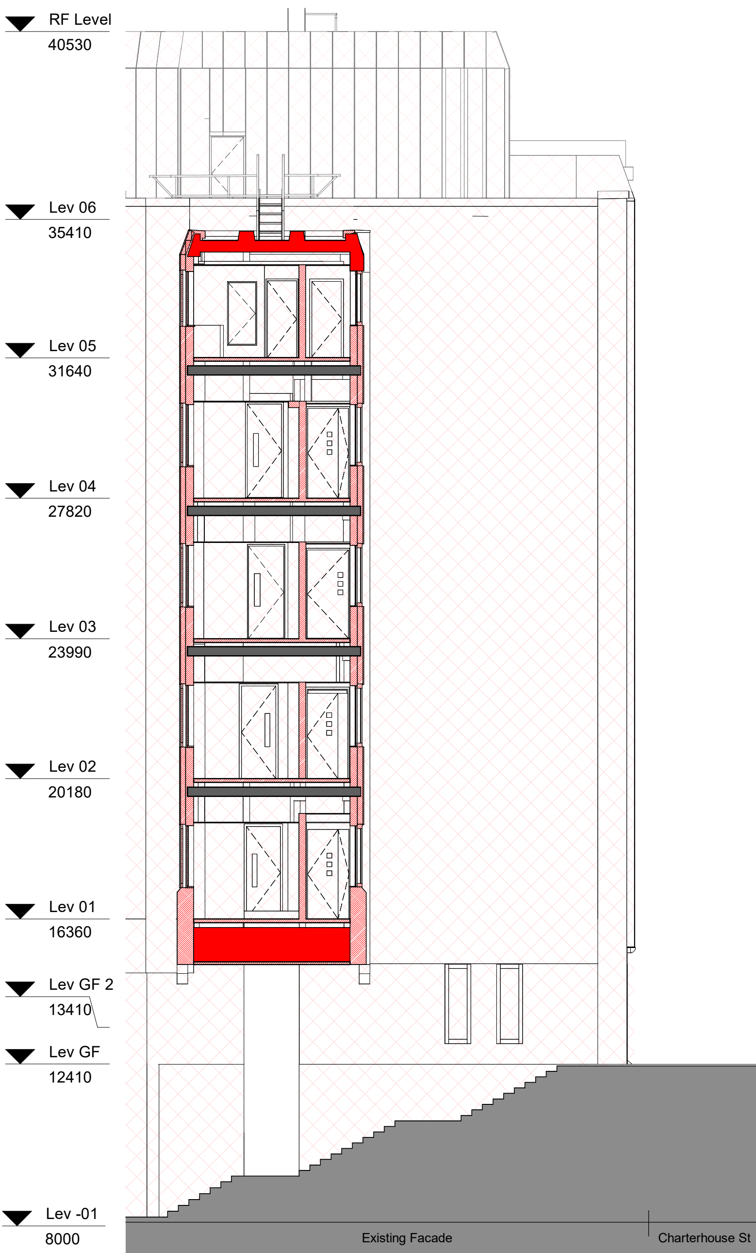
① Demolition Elevation West - SH Bridge 1 : 100
