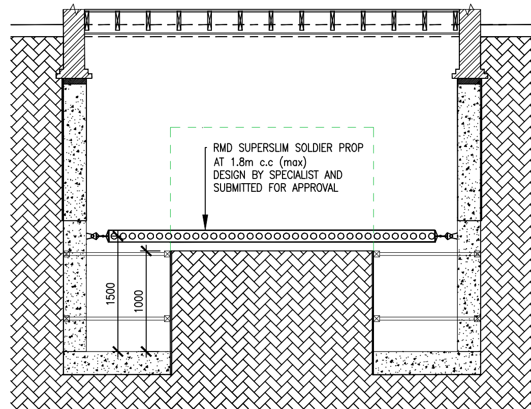
STAGE 7 – REDUCE GROUND AND INSTALL LOWER PROP
