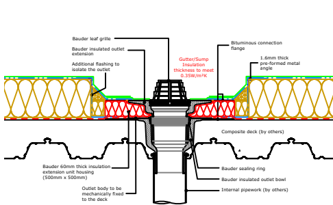
ROOF OUTLET DETAIL
