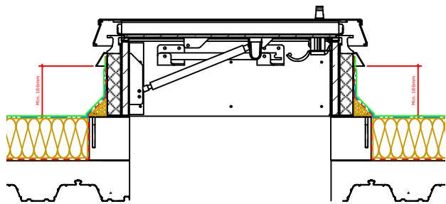
ROOF HATCH DETAIL
