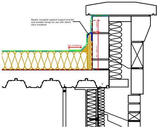
INSULATED PARAPET UPSTAND DETAIL refer to Hale Brown drawing 430(ED)403 - detail 2
