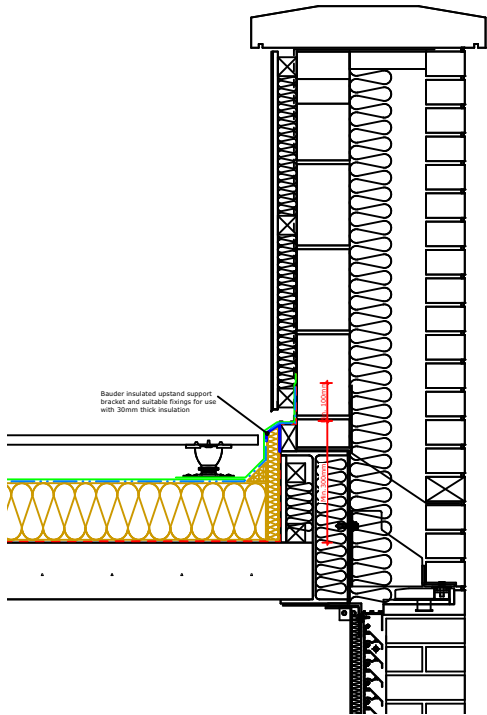
INSULATED UPSTAND DETAIL refer to Hale Brown drawing 430(ED)412 - detail 1
