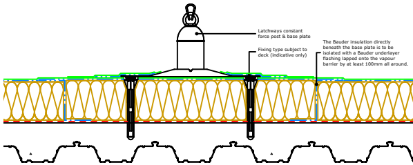
LATCHWAYS CONSTANT FORCE POST DETAIL
