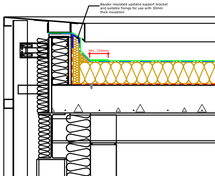
STUDWORK PARAPET UPSTAND DETAIL refer to Hale Brown drawing 430(ED)424 - details 1 & 2
