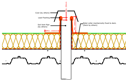
SOIL VENT PIPE DETAIL
