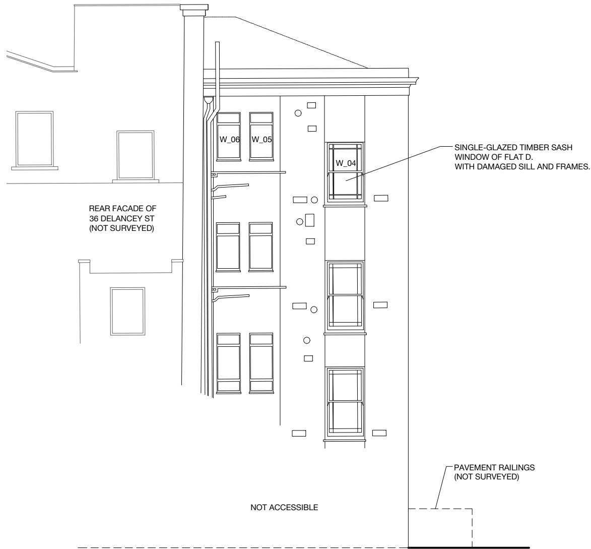
01 EXISTING NORTH-WEST ELEVATION 00B-03 SCALE 1:100
