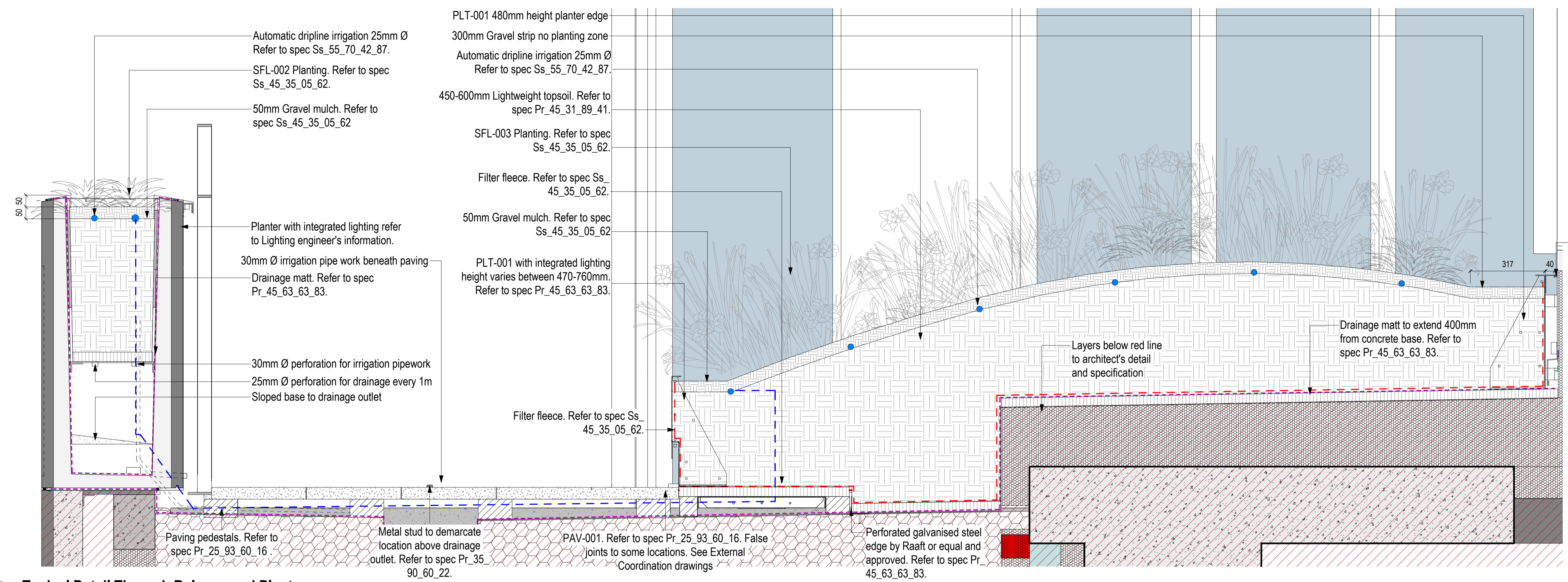
1 Typical Detail Through Balcony and Planter 1:10
