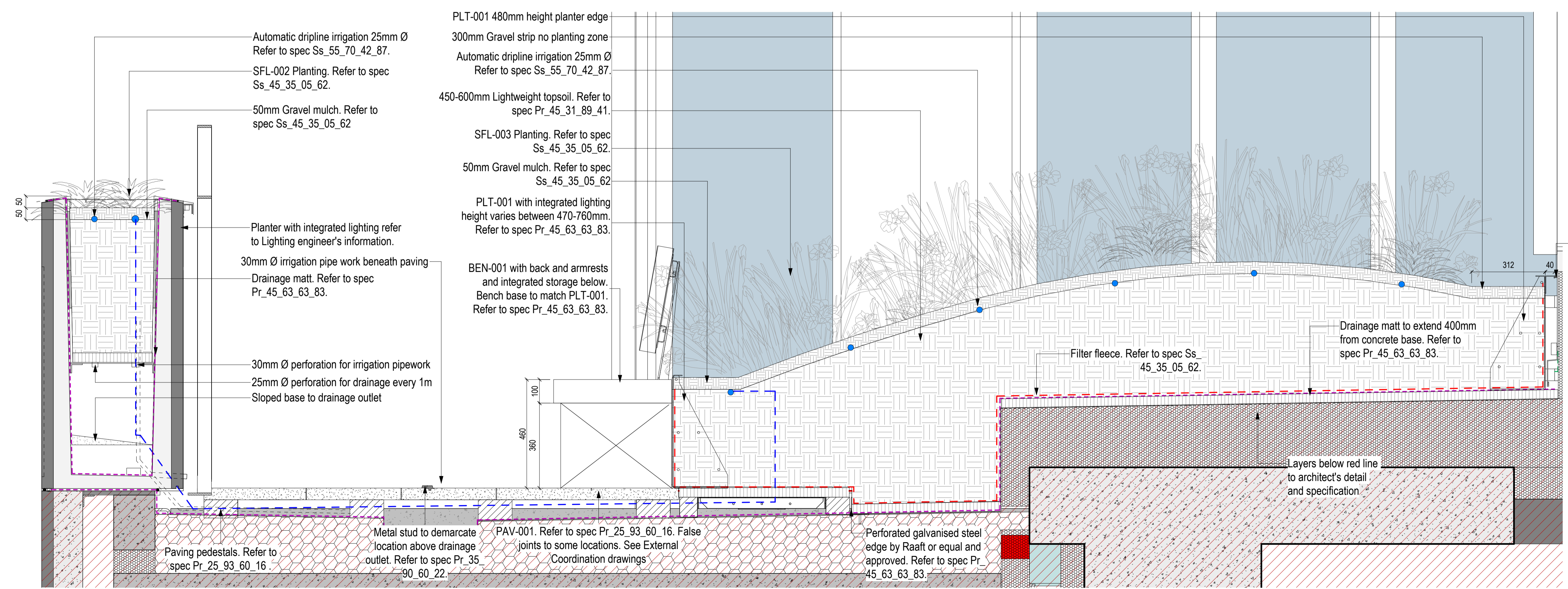
2 Typical Detail Through Balcony, Bench and Planter 1:10
