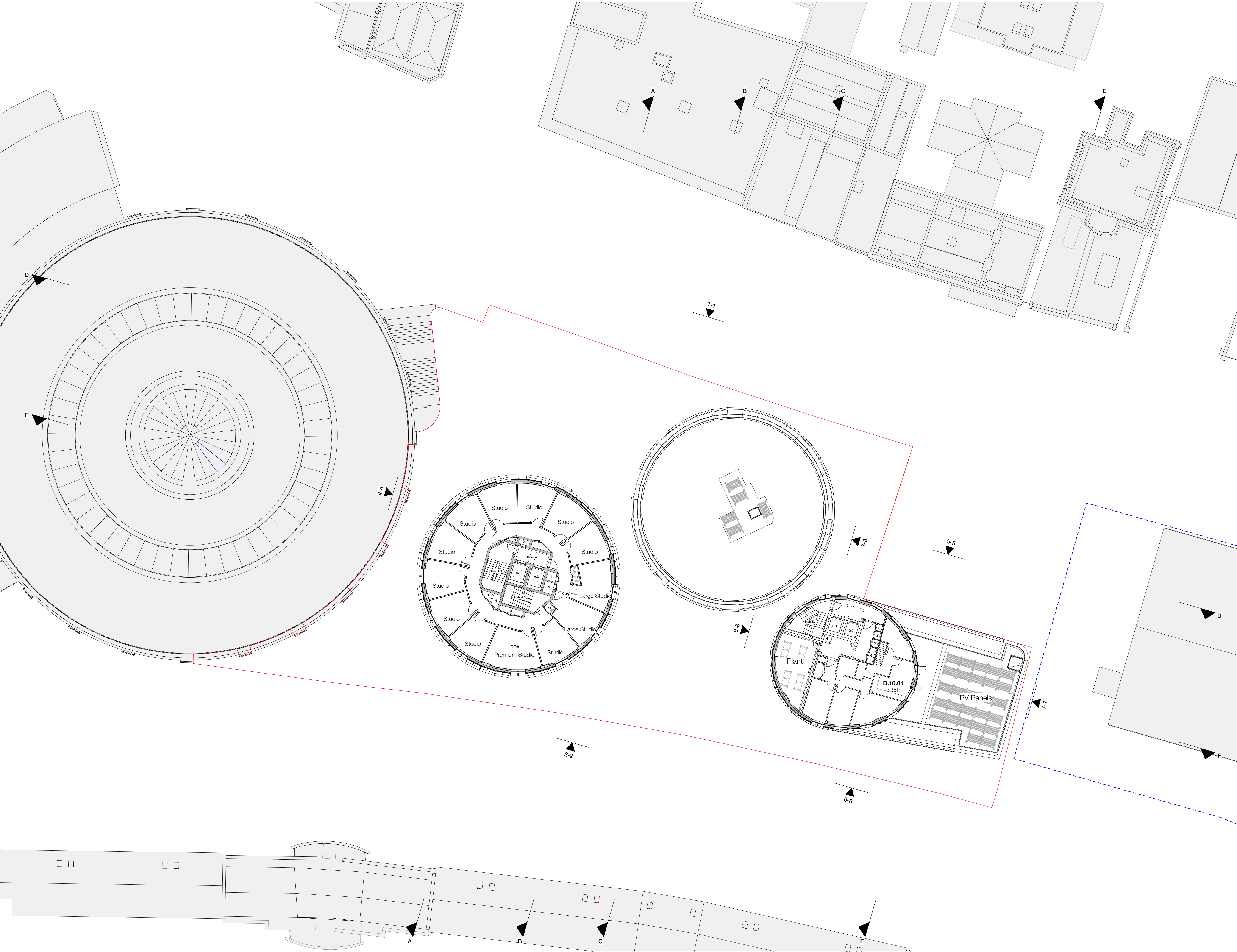
1 Level 10 Floor Plan 1 : 200
