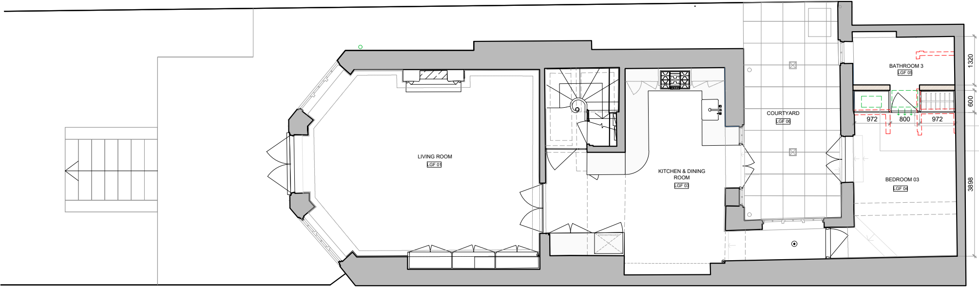
LOWER GROUND FLOOR PLAN
