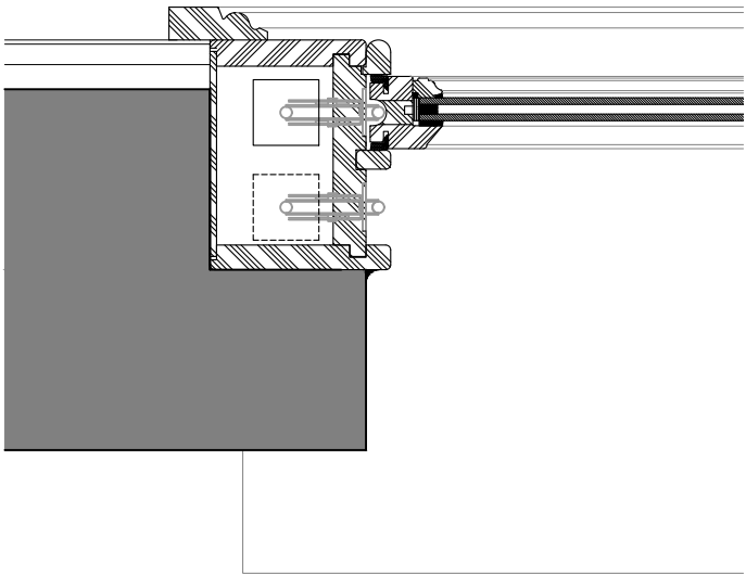
SECTION B-B – 1:5
