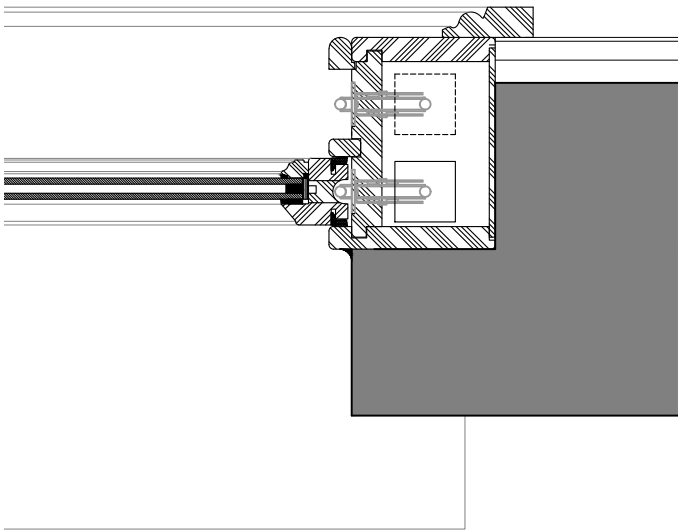
SECTION C-C – 1:5
