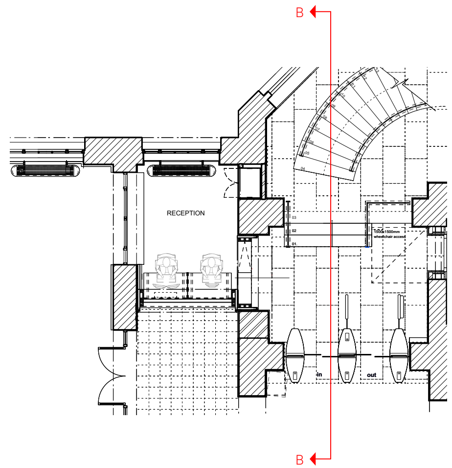
2 Key Plan Showing Section Cut 1:100 @ A1 / 1:200 @ A3
