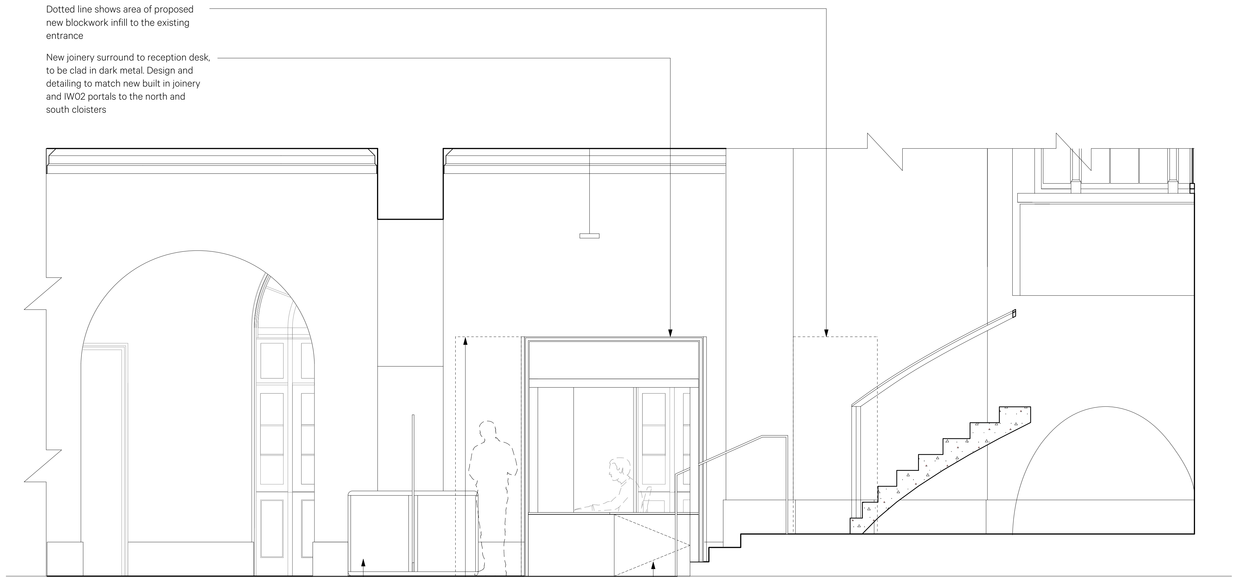
1 Proposed Elevation B 1:25 @ A1 / 1:50 @ A3
