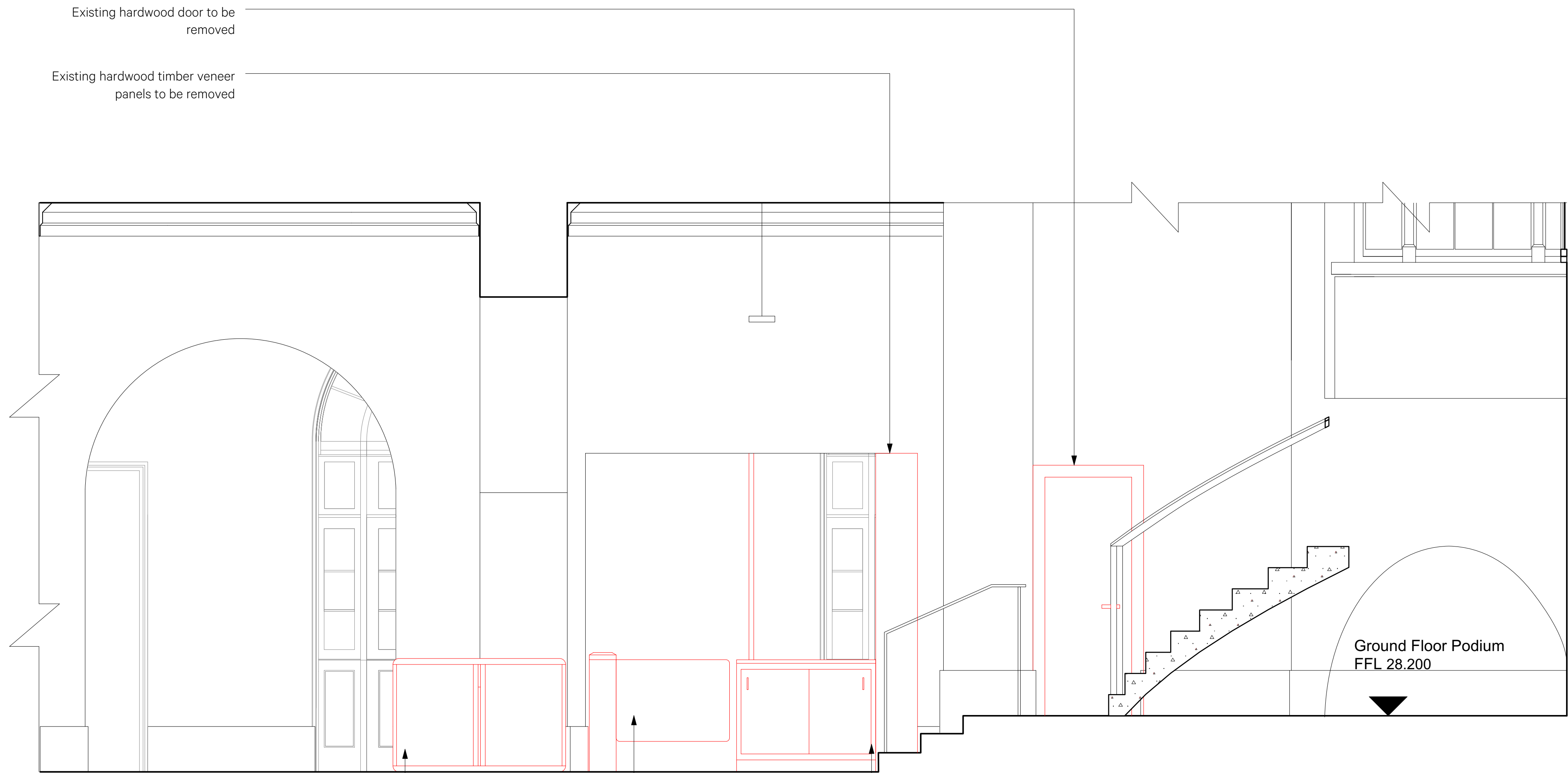
1 Fabric Removal Elevation B 1:25 @ A1 / 1:50 @ A3
