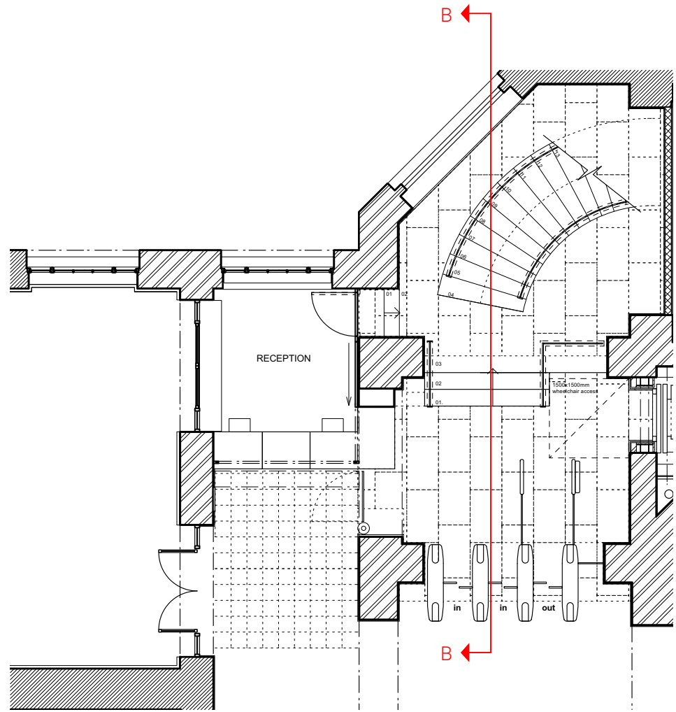
2 Key Plan Showing Section Cut 1:100 @ A1 / 1:200 @ A3
