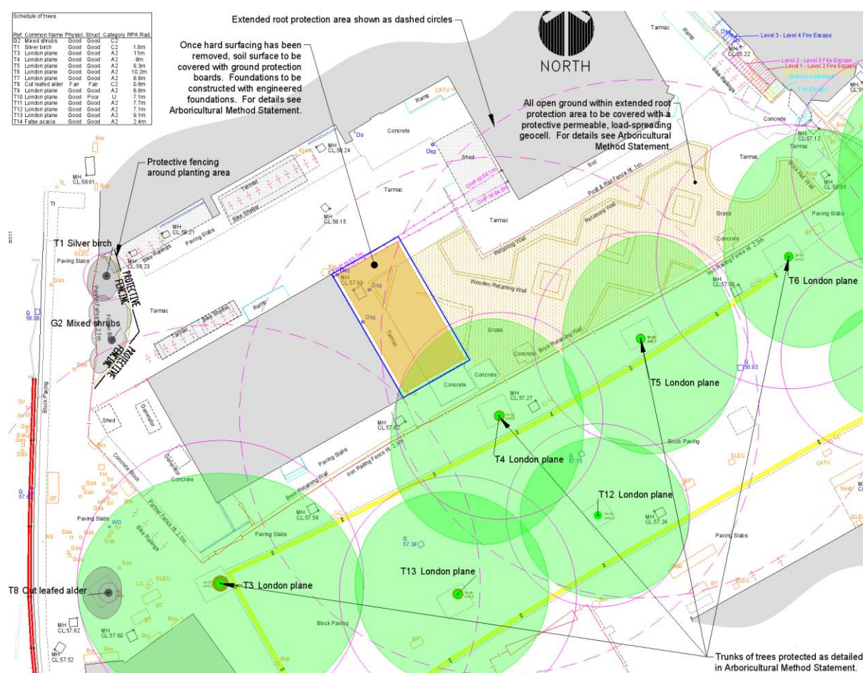
Extract from the tree protection plan showing position of ground protection.
