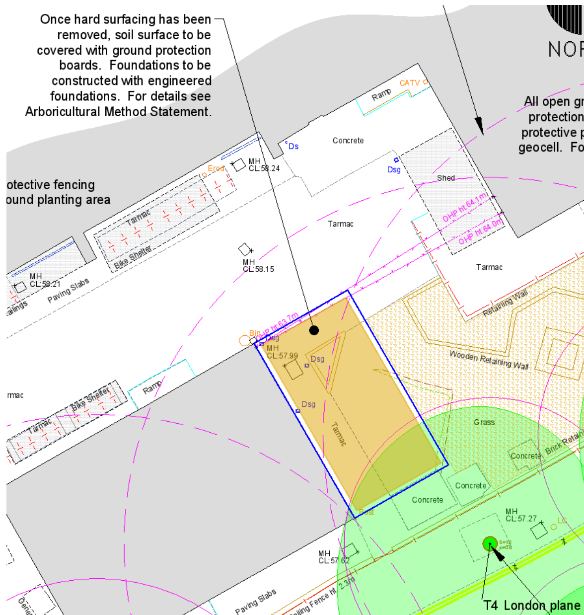
Details of ground protection from tree protection plan.
