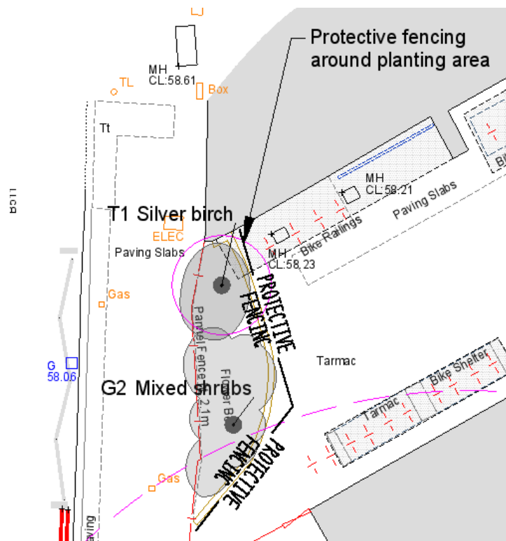
Extract from tree protection plan showing position of protective fencing.
