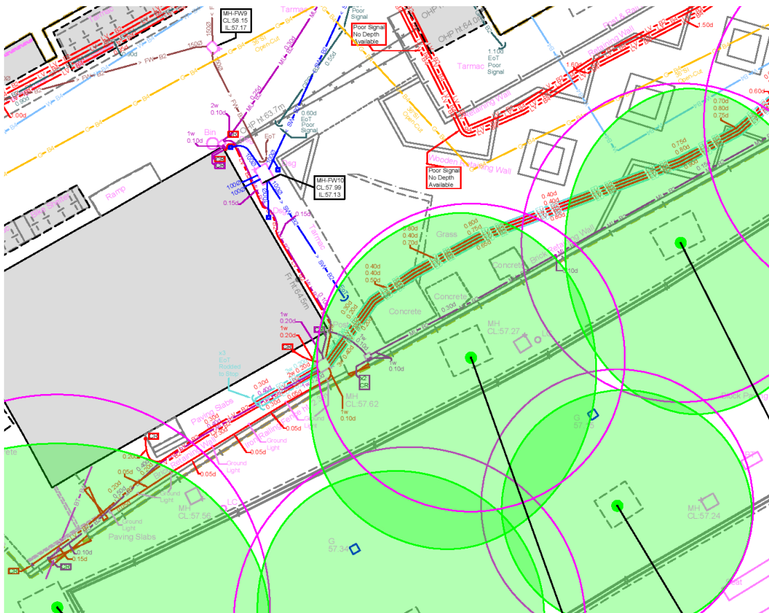
Section of plan showing underground utilities.
