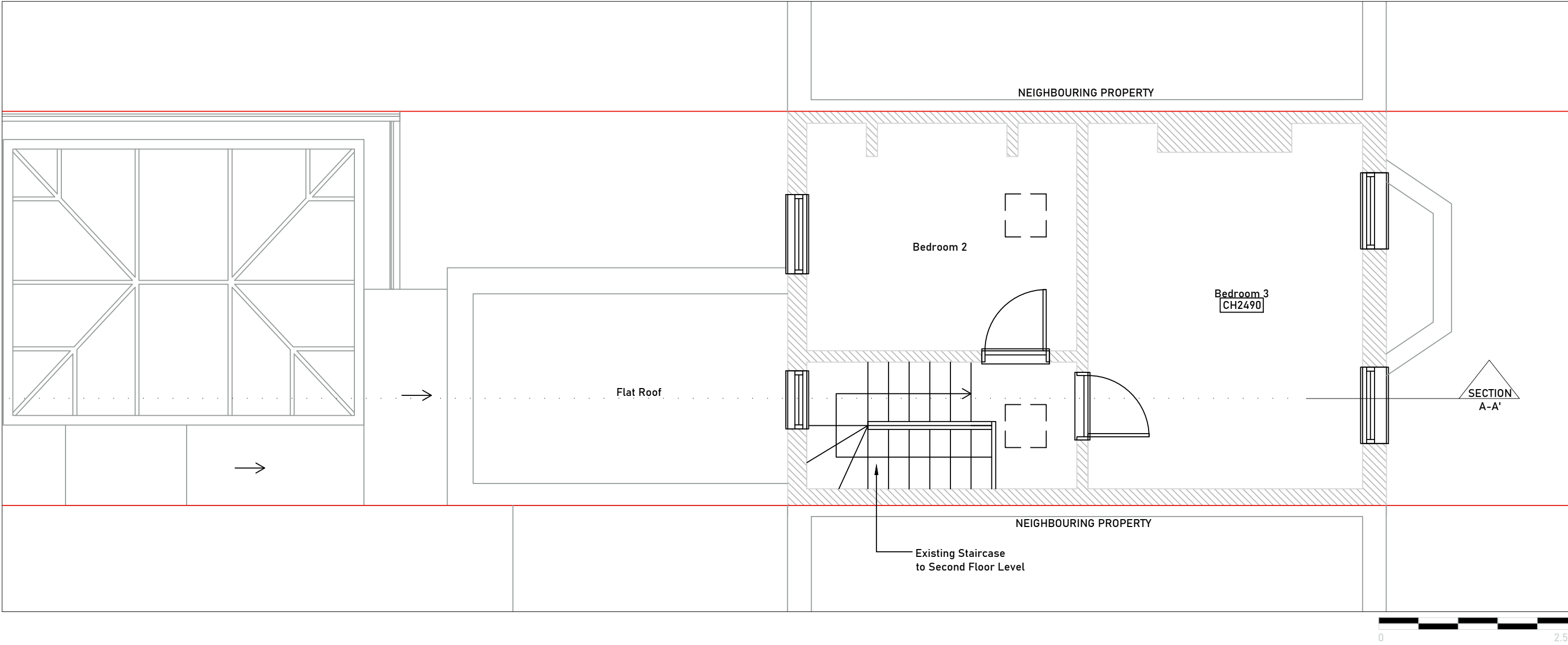
[01] EXISTING SECOND FLOOR PLAN
