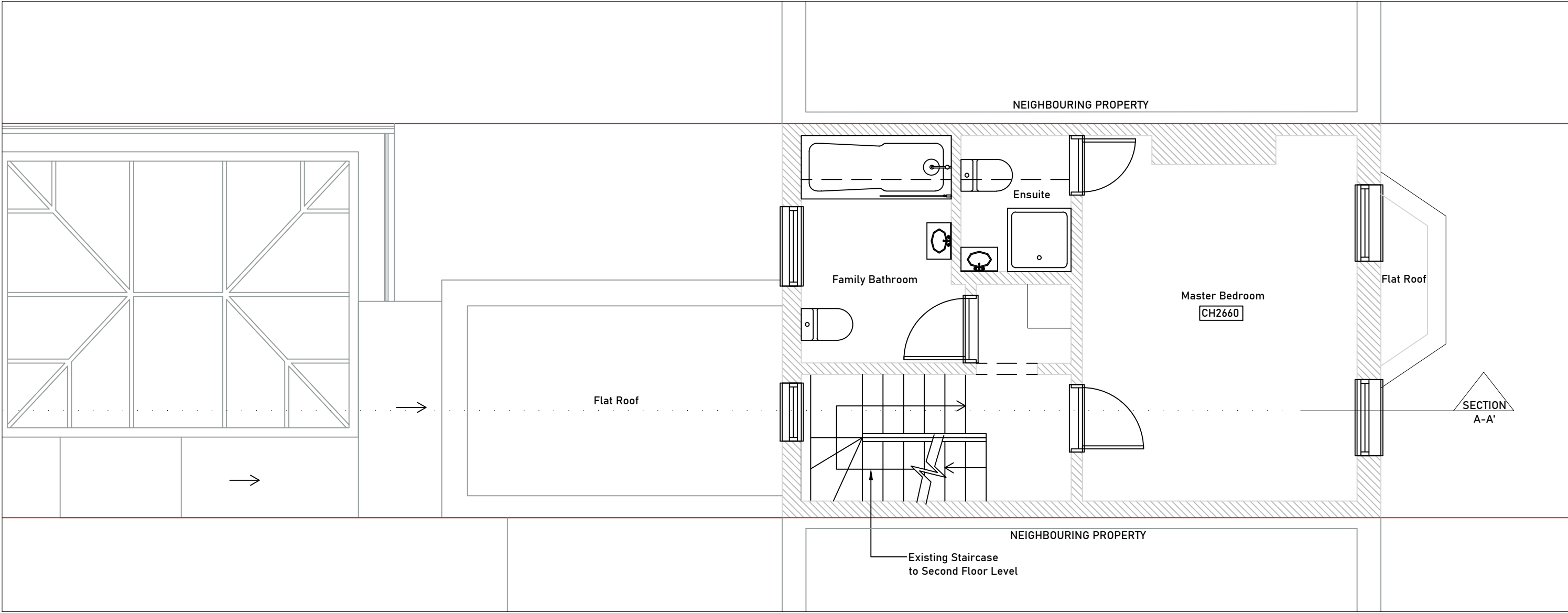
[01] EXISTING FIRST FLOOR PLAN
