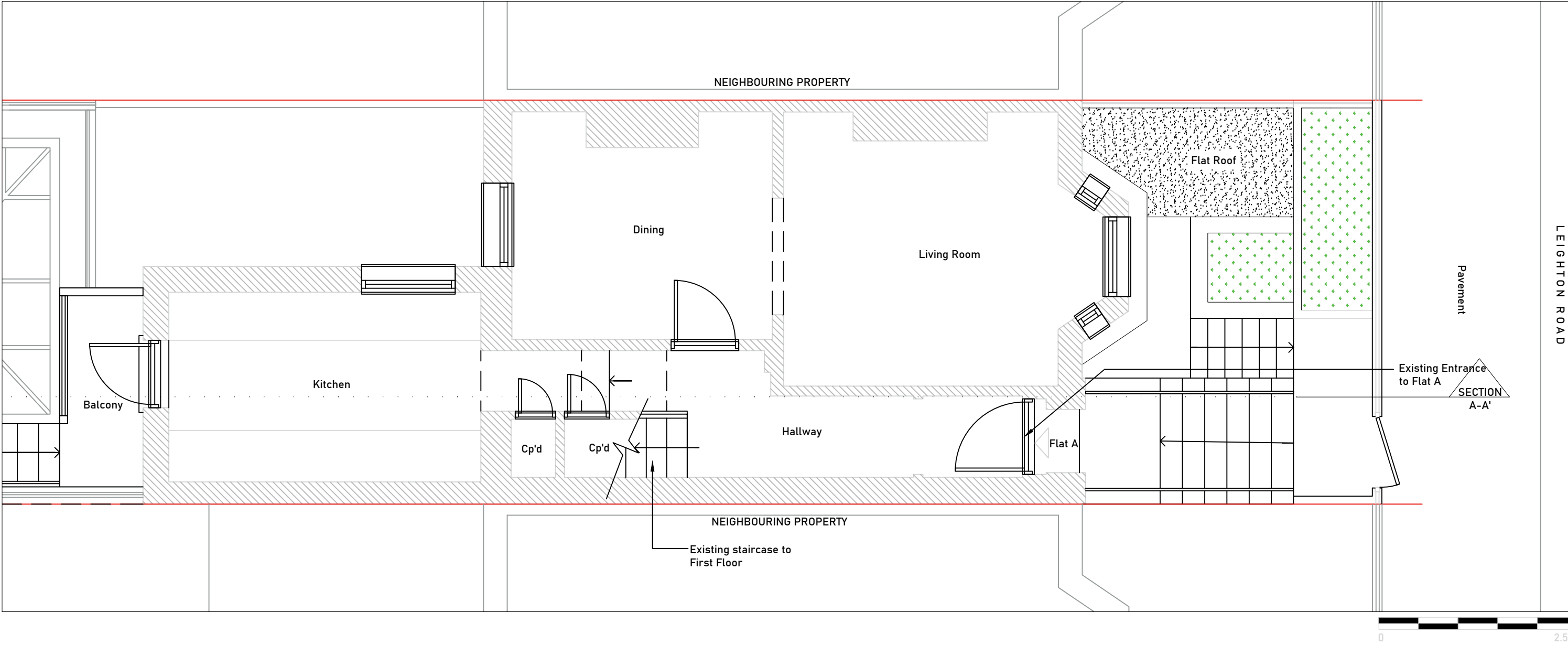
[01] EXISTING GROUND FLOOR PLAN
