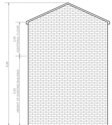
PROPOSED SIDE ELEVATION 2 SCALE 1:100 @ A3
