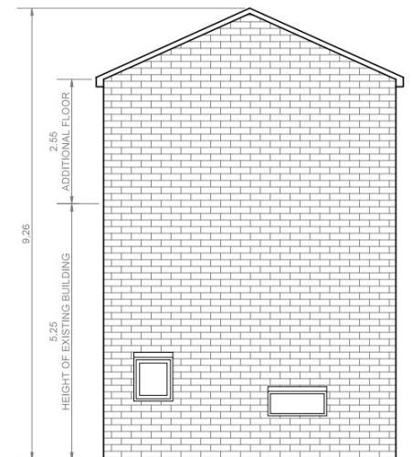
PROPOSED SIDE ELEVATION 1 SCALE 1:100 @ A3
