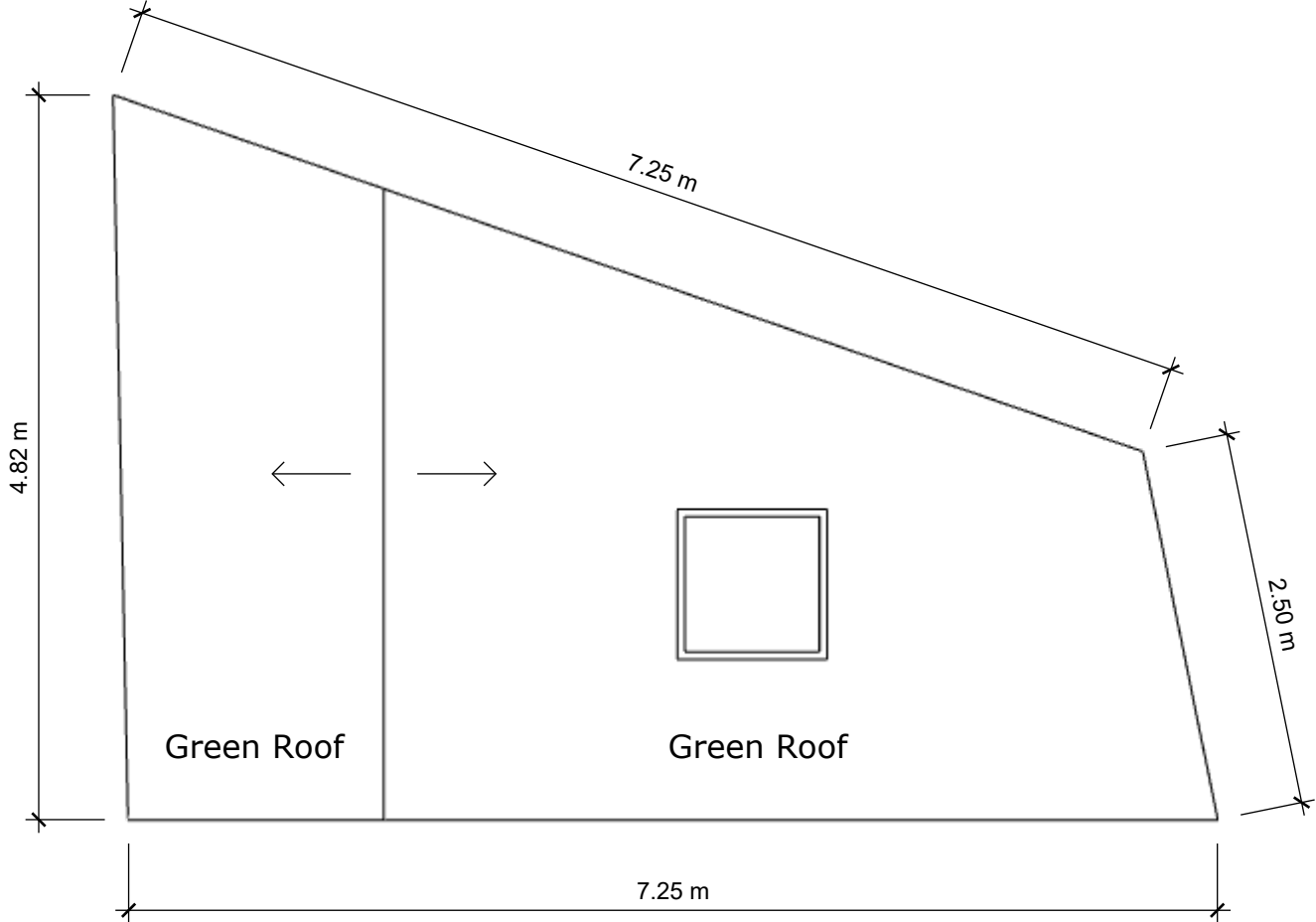
Roof Plan
