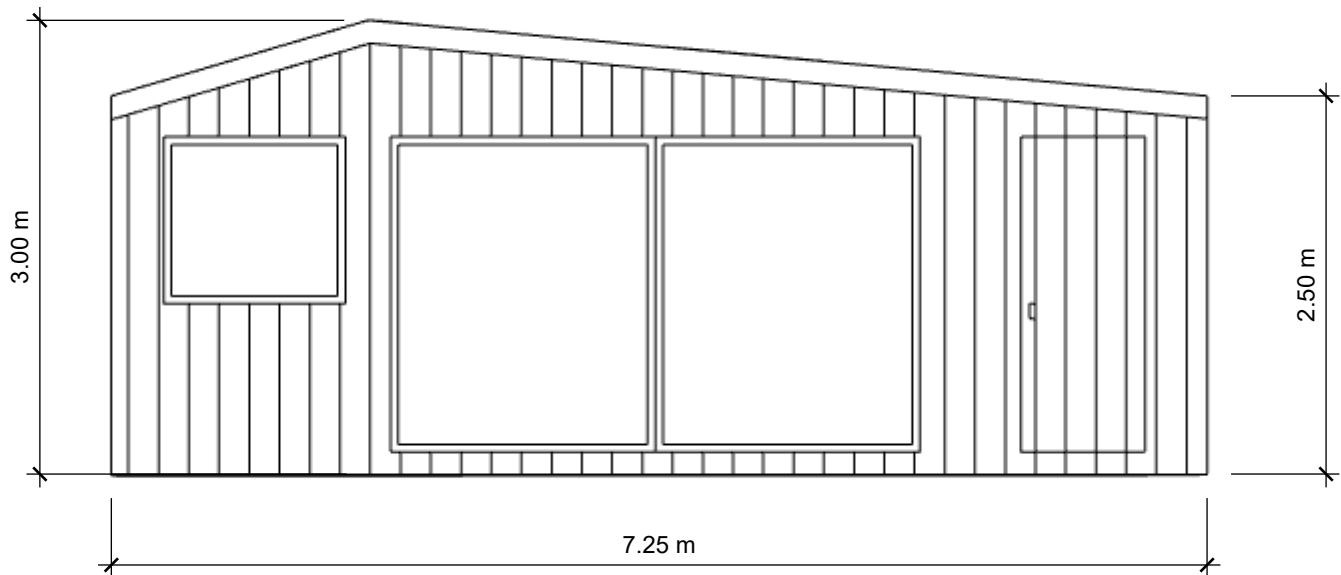
North Elevation
