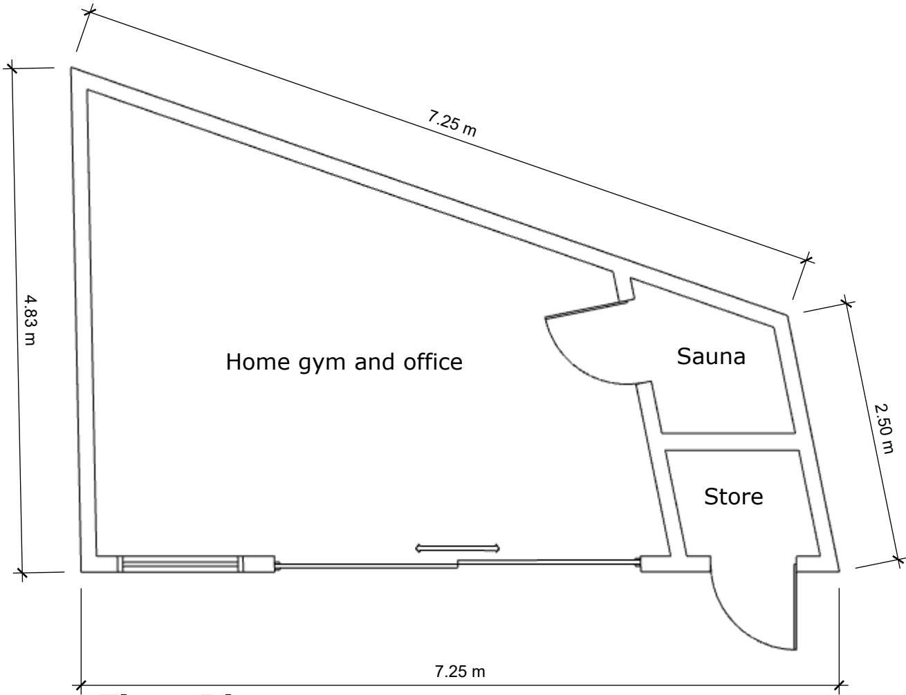
Floor Plan
