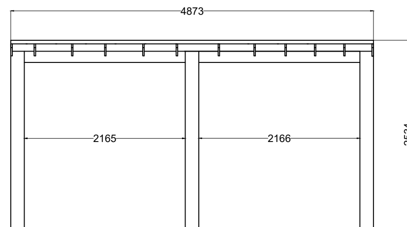
Proposed Pergola Front Elevation
