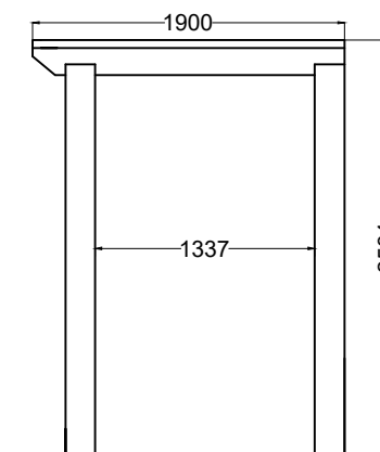
Proposed Pergola Side Elevation
