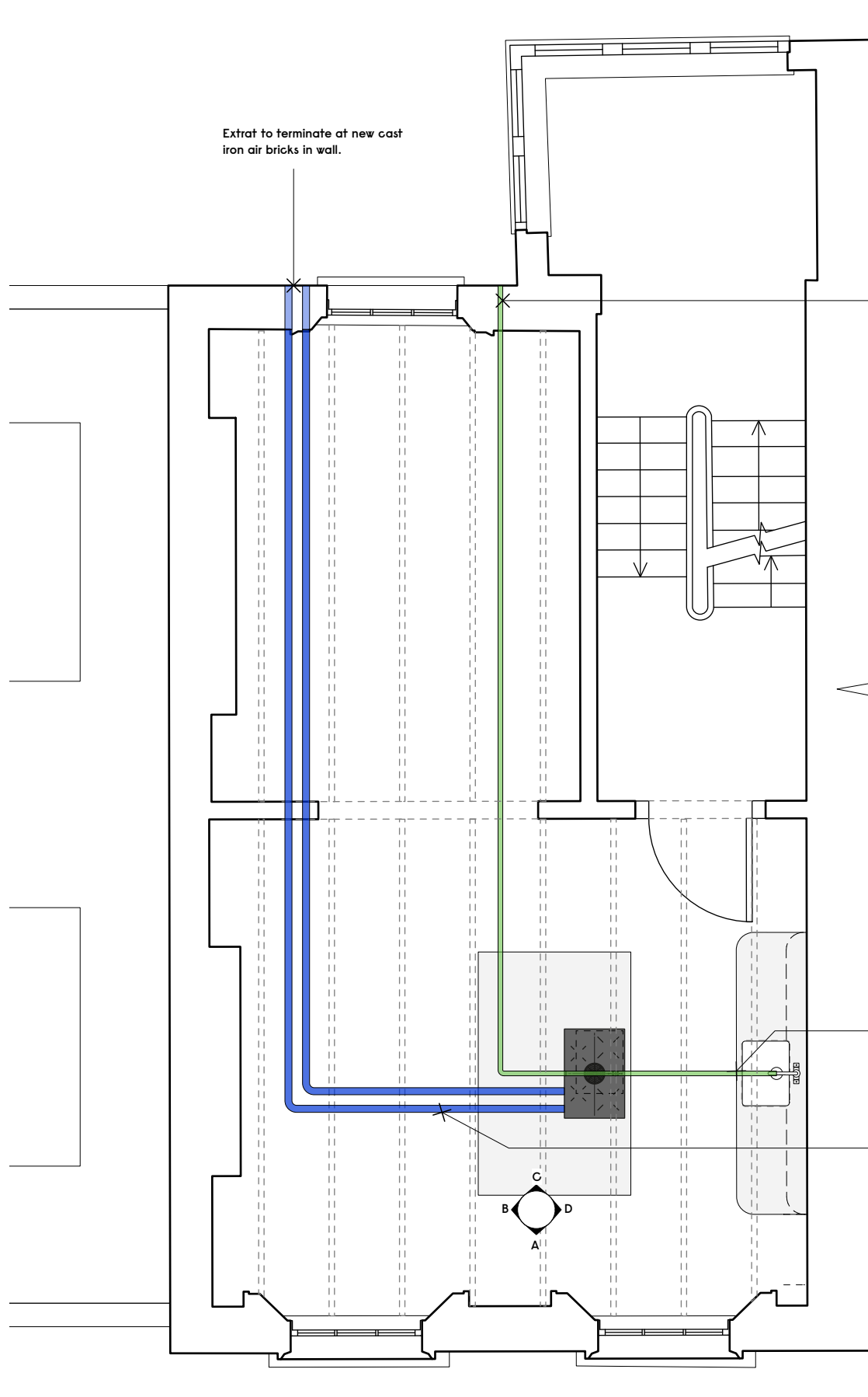
1 Proposed Plan Scale: 1:50
